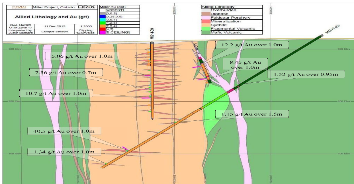
Figure 0-2 Geological cross section through the Allied Syenite (from Hart, 2015).
