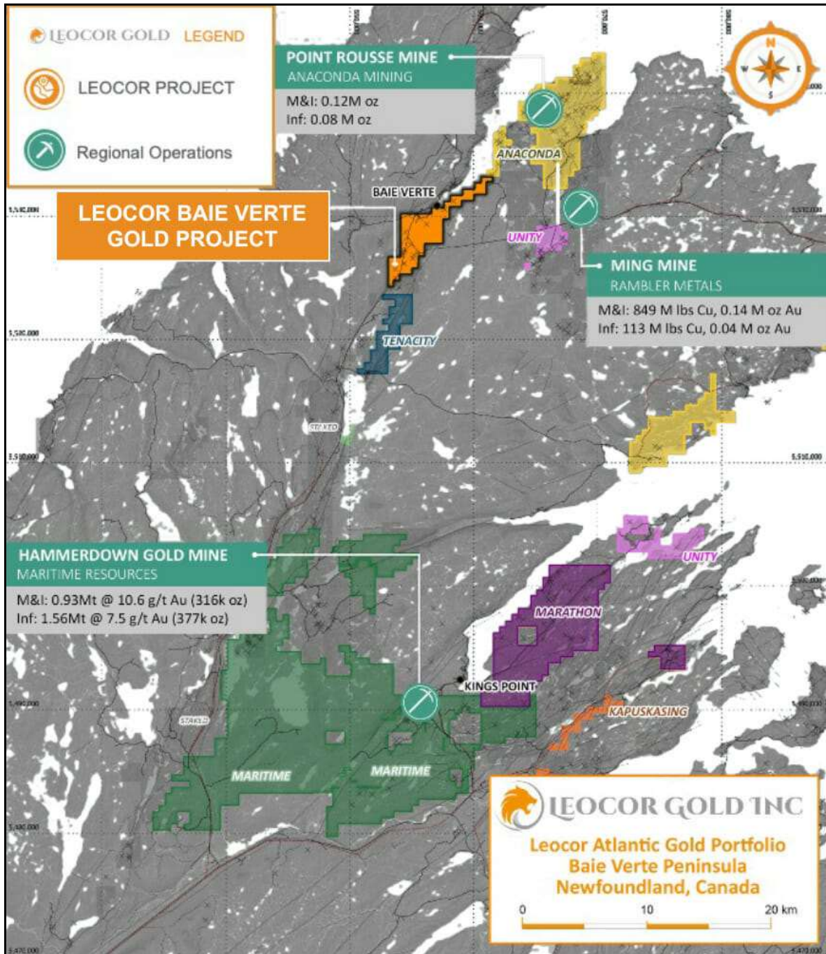
Figure 3: Location of the Baie Verte Project (Dorset), Newfoundland, Canada
