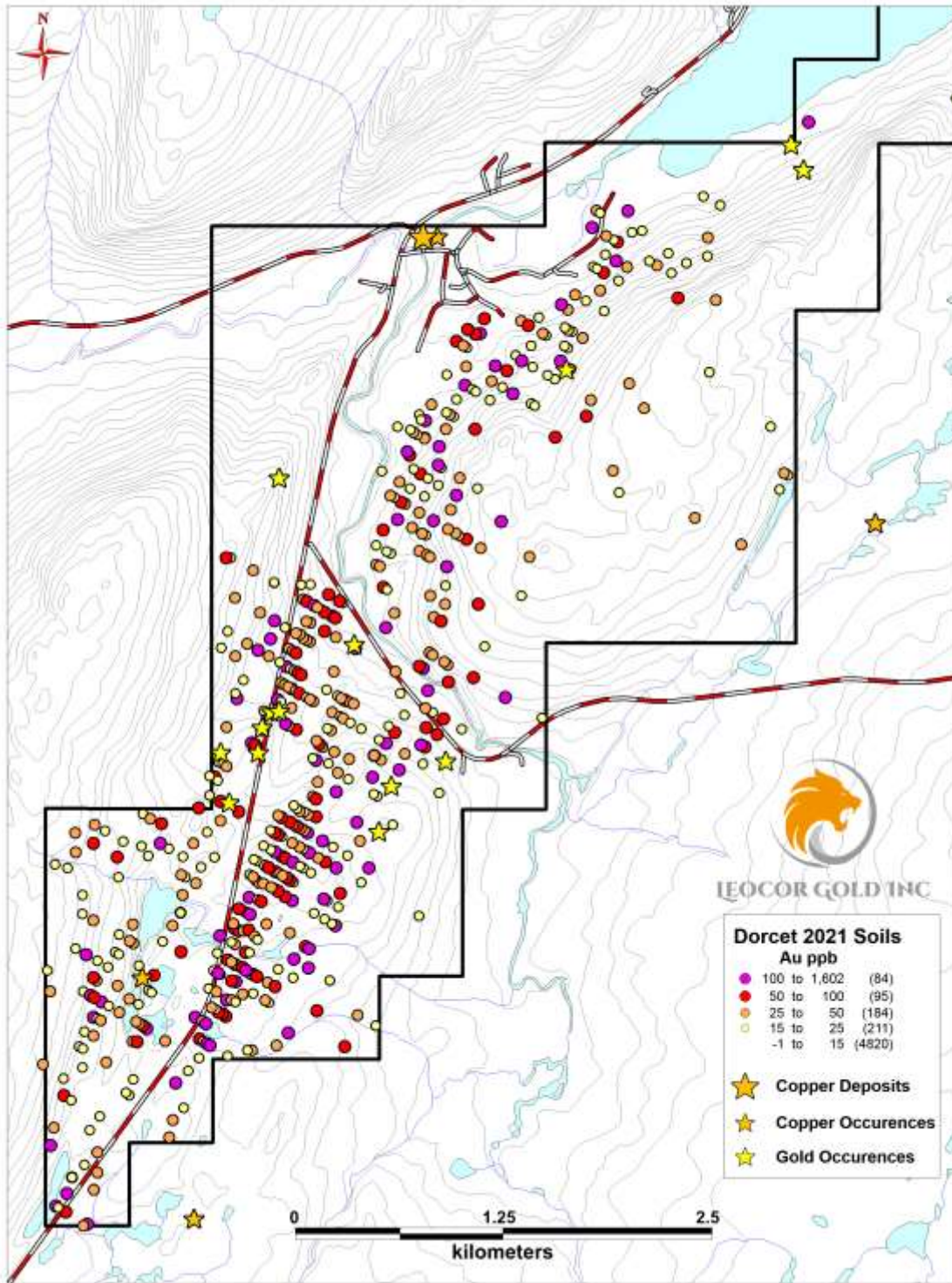
Figure 1: Gold-in-soil results, Baie Verte project (Dorset and adjacent projects), Newfoundland, Canada
