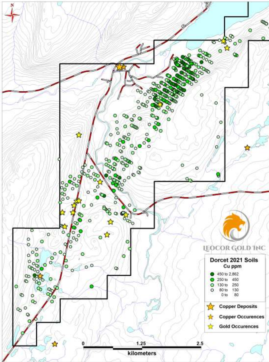
Figure 2: Copper-in-soil results, Baie Verte project (Dorset and adjacent projects), Newfoundland, Canada
