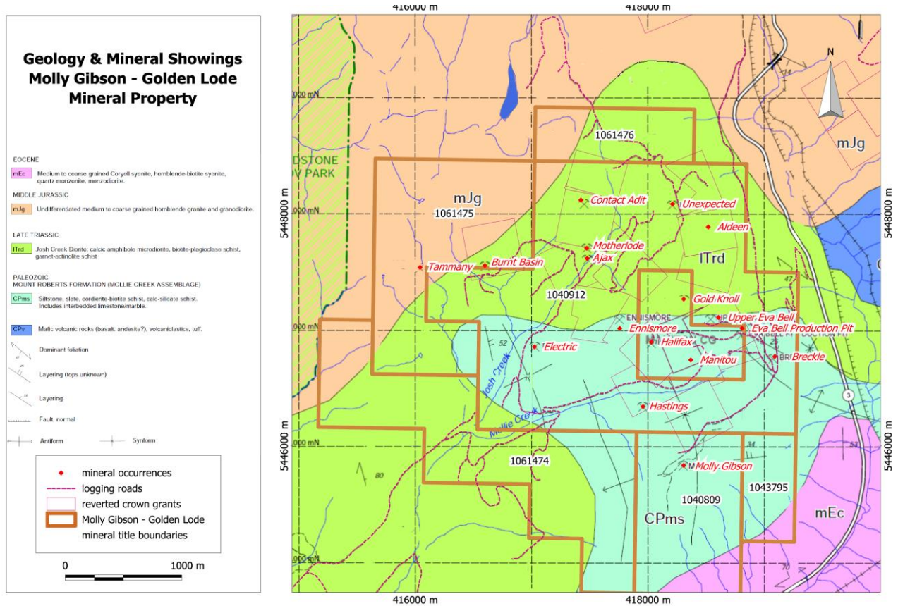
Figure 6. Property geology and location of mineral occurrences. Map prepared by D.G. MacIntyre, November 2018. Base map from Caron (2008).
