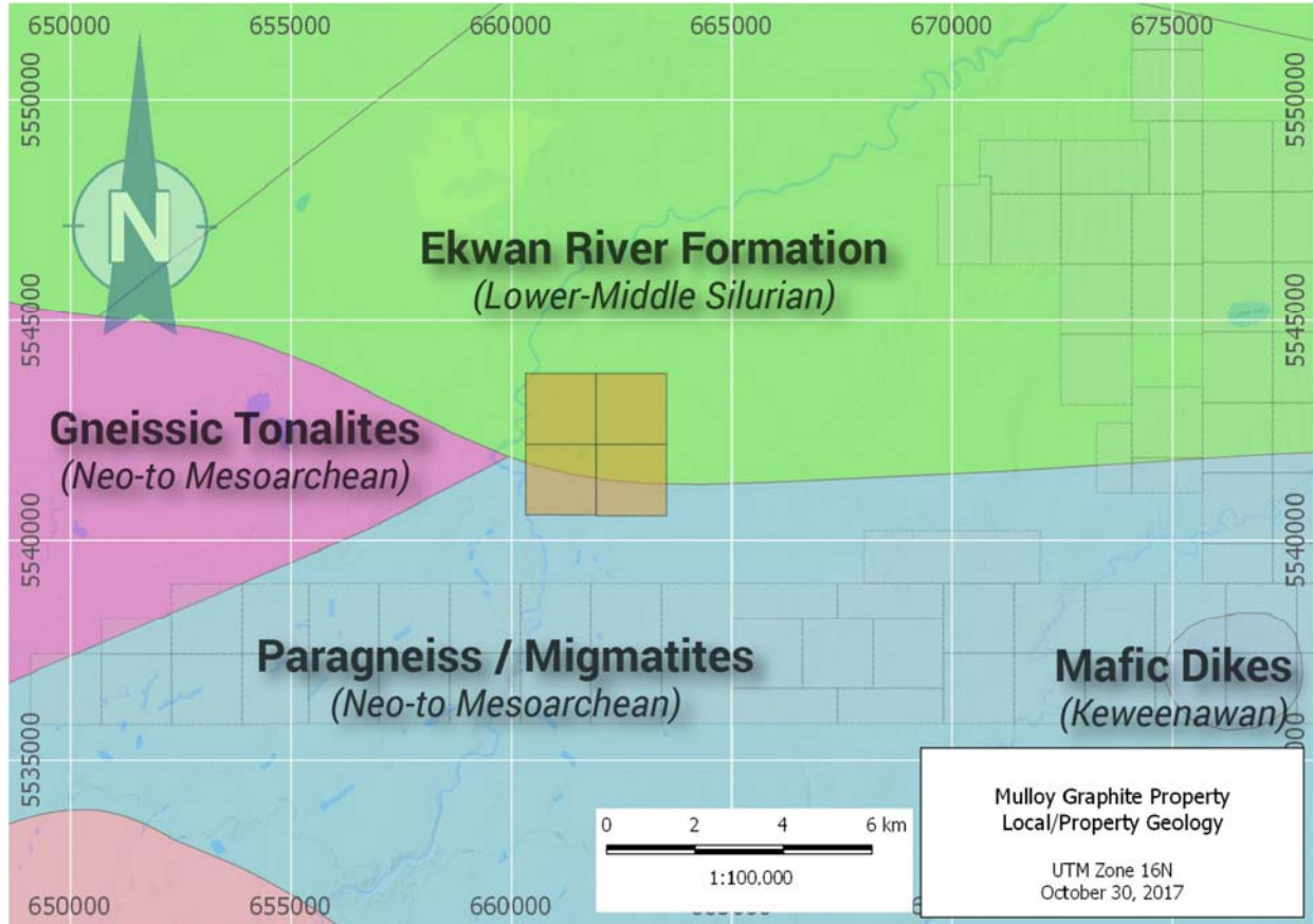
Figure 7: Local Geology
