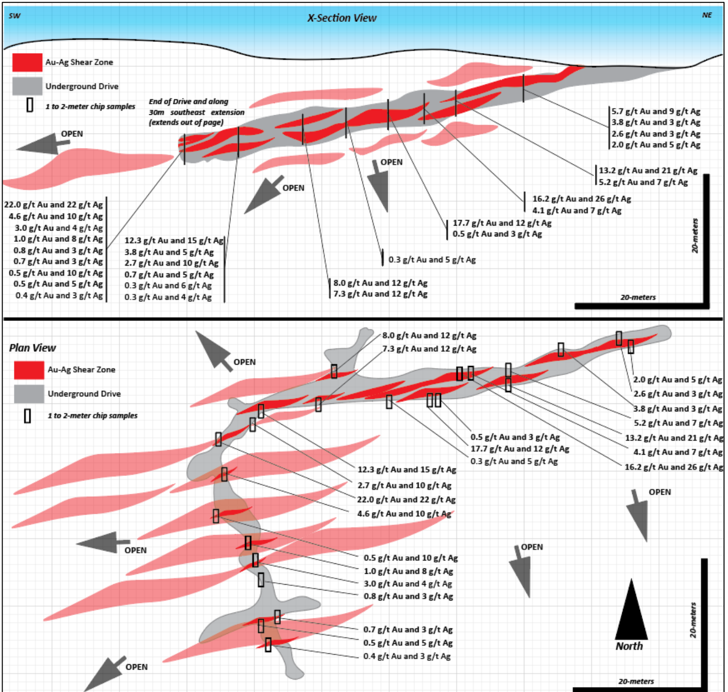
Figure 2. Plan view and X-Section of the San Ramon Underground Drive. High-grade mineralization is open at depth and along strike.
