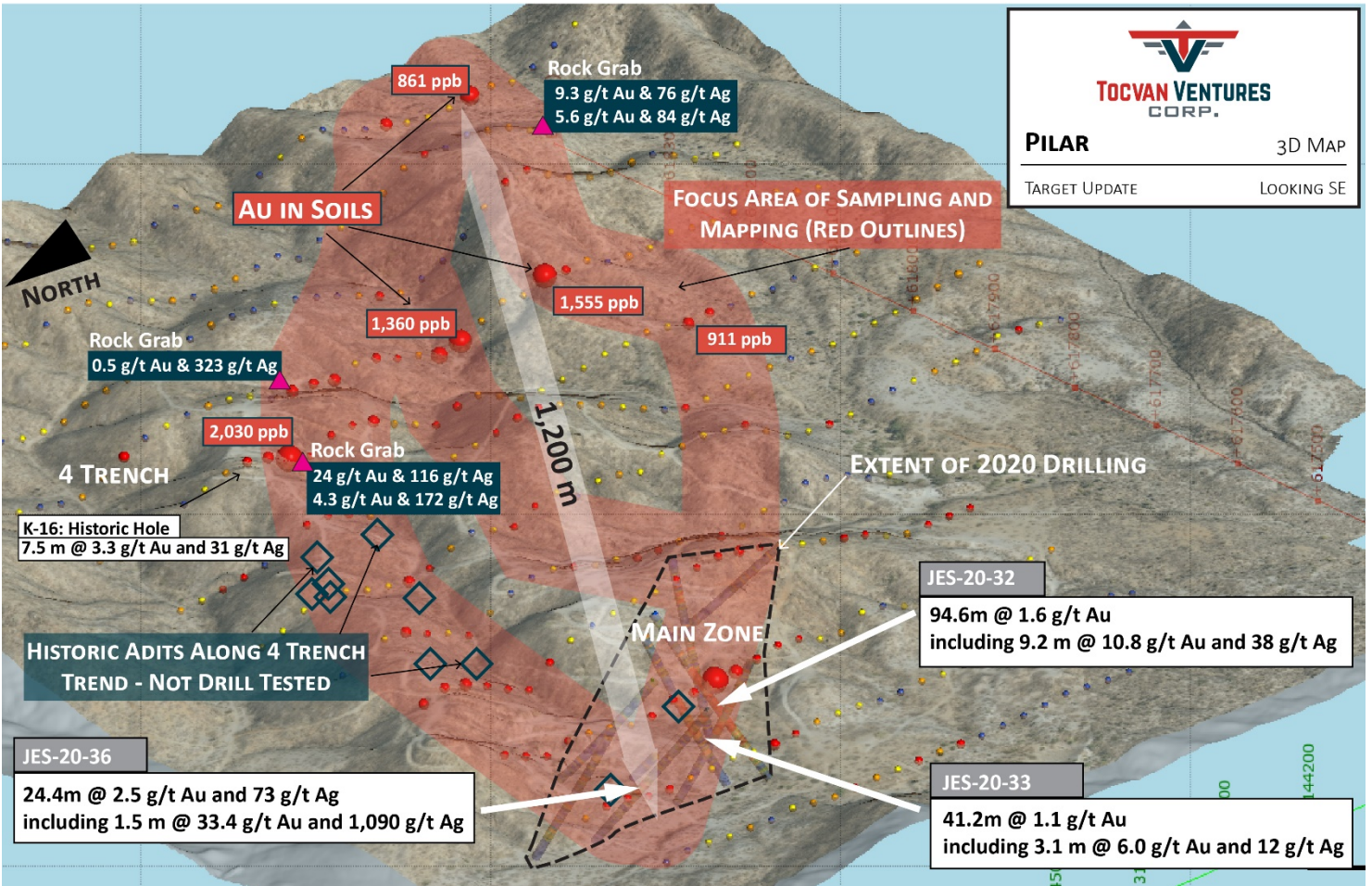
Figure 1. 3D Target Map of Pilar Gold-Silver Project. Outside of the Main Zone the majority of the project area has not been drill tested.
