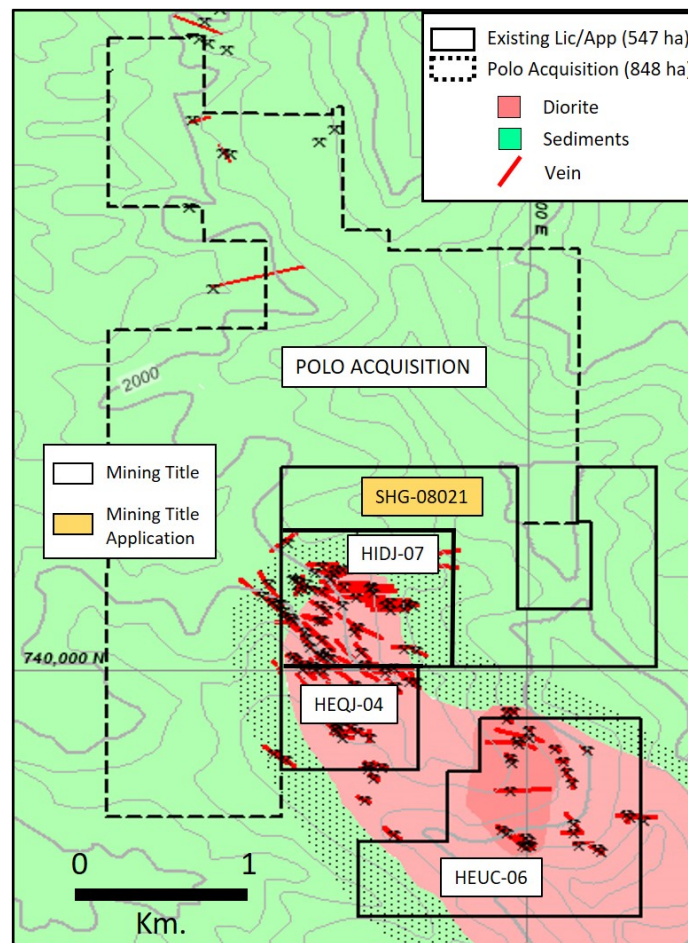
Figure 1. Mining licenses, applications and known vein-type occurrences in the project area as of August 31, 2021.
