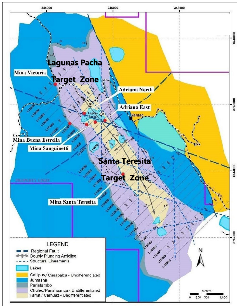
Figure 7.3 Property Geology Map and Local Prospects
