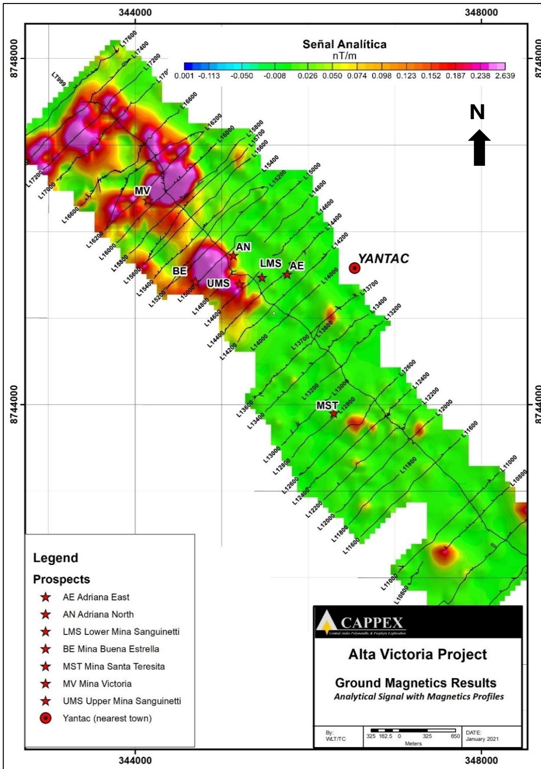
Figure 9.3 Ground Magnetism Survey Invalid source specified.
