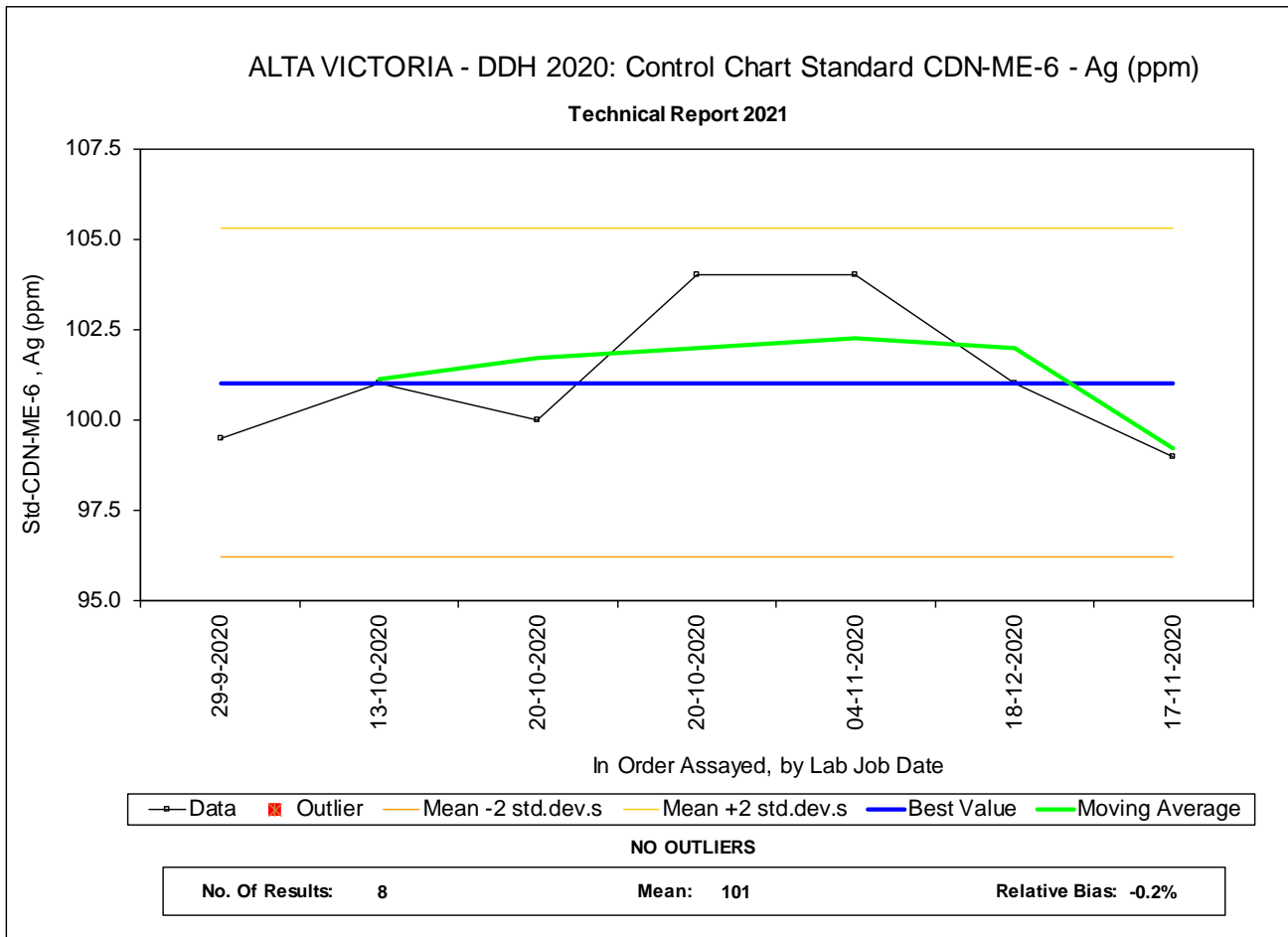
Figure 11.2 Standard CDN-ME-6 for Ag (ppm) – Drilling Program 2020
