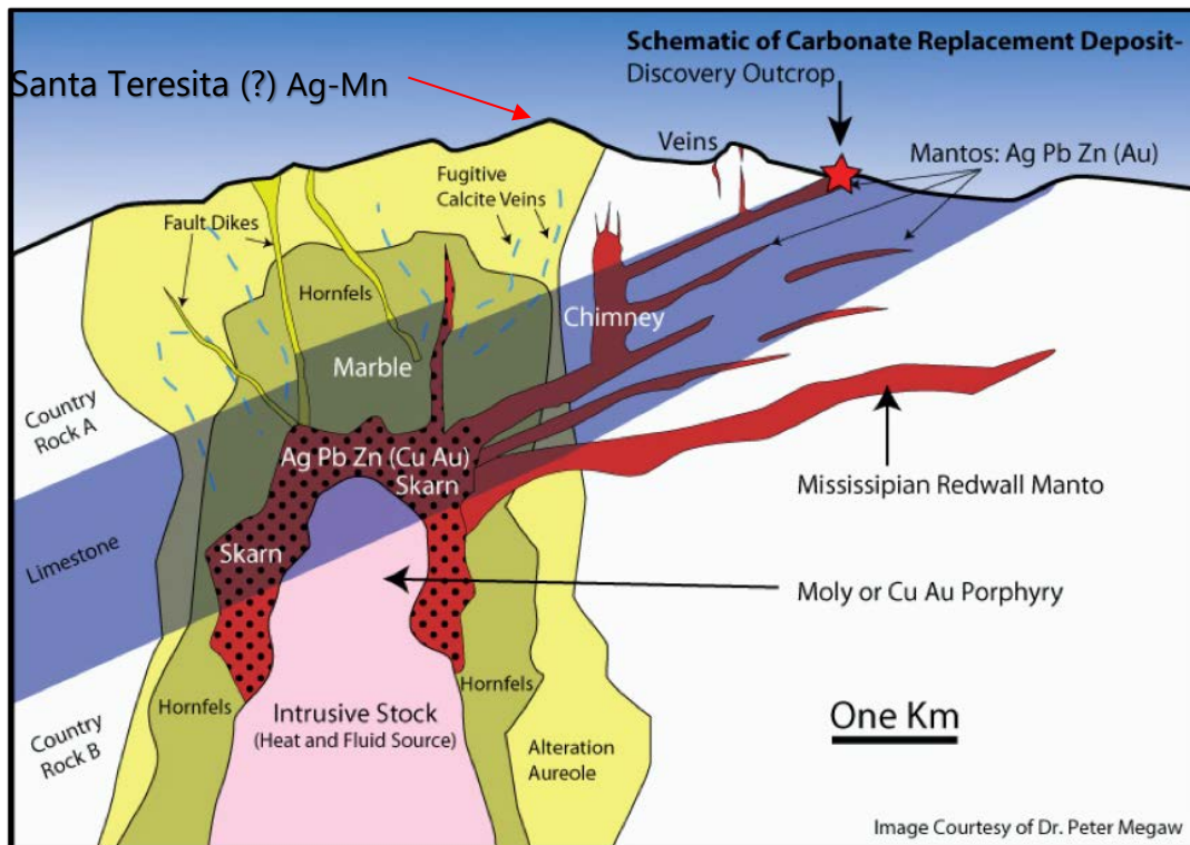
Figure 8.1 Schematic section of Carbonate Replacement Deposit (CRD) Invalid source specified.
