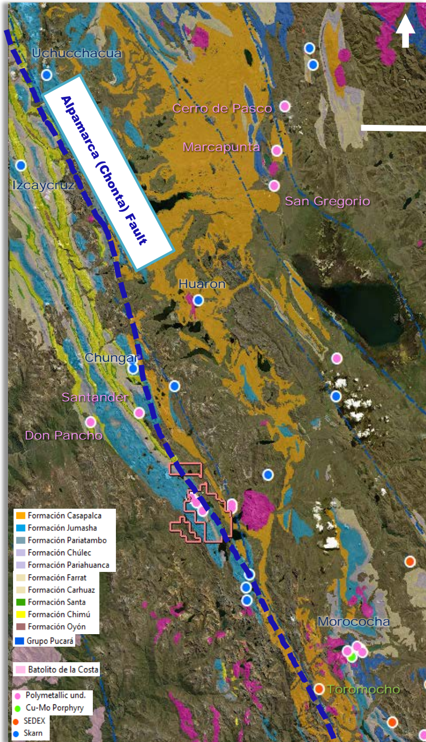
Figure 7.1 Regional Geological Map & Principal Mines
