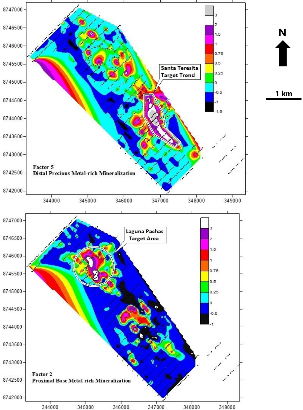
Figure 9.1 Principal Component Factor Analysis MapsInvalid source specified.
