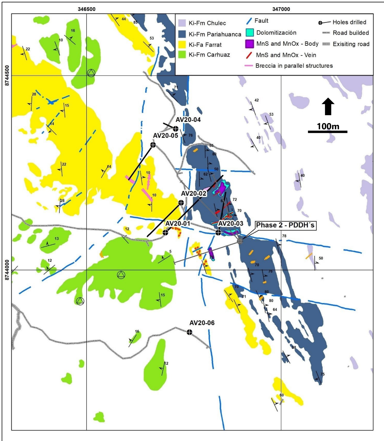
Figure 10.2 Detailed Geological Map of the Santa Teresita Target with Completed Scout Drill Holes and Proposed Drill Holes
