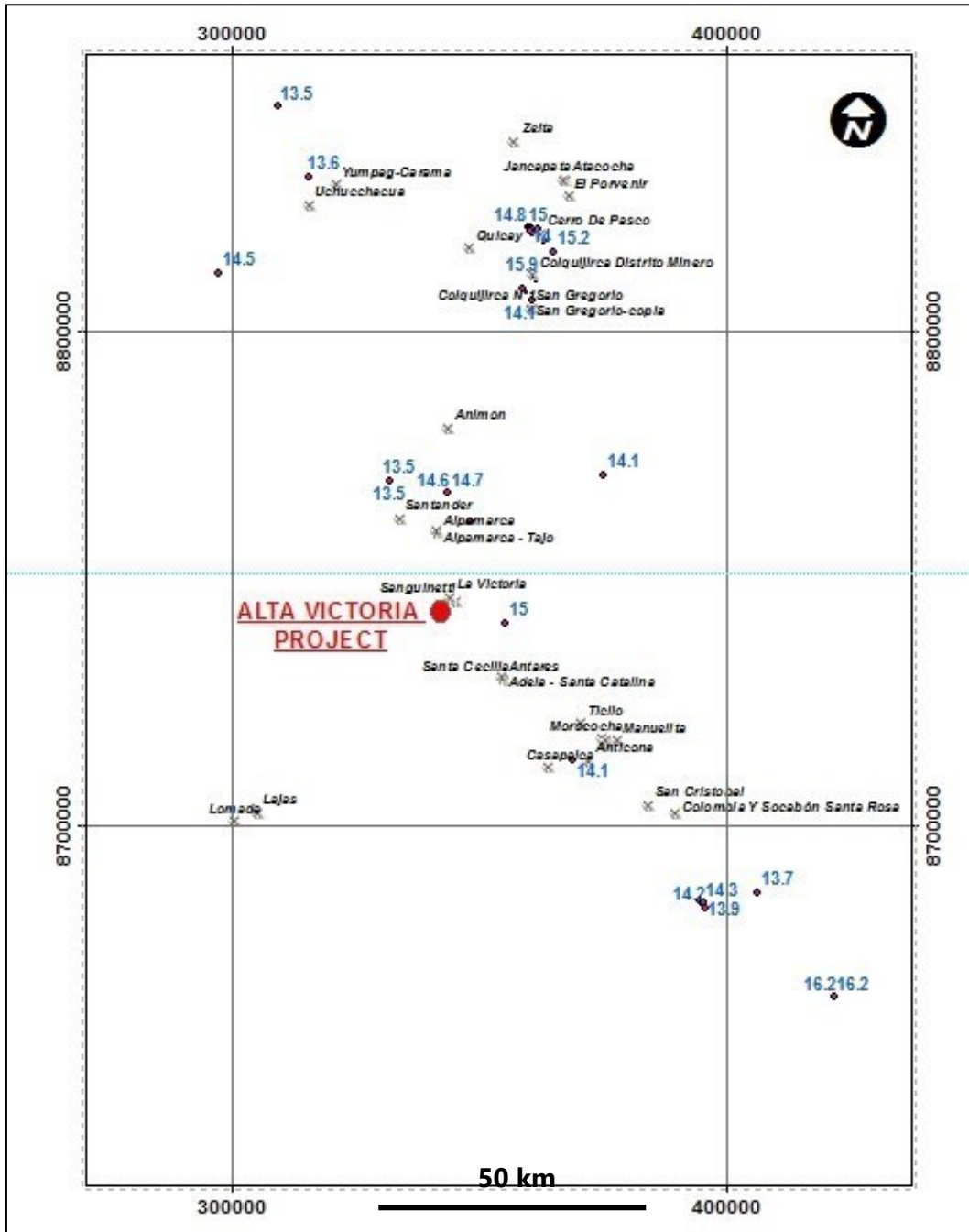
Figure 7.2 District age dates of igneous rocks
