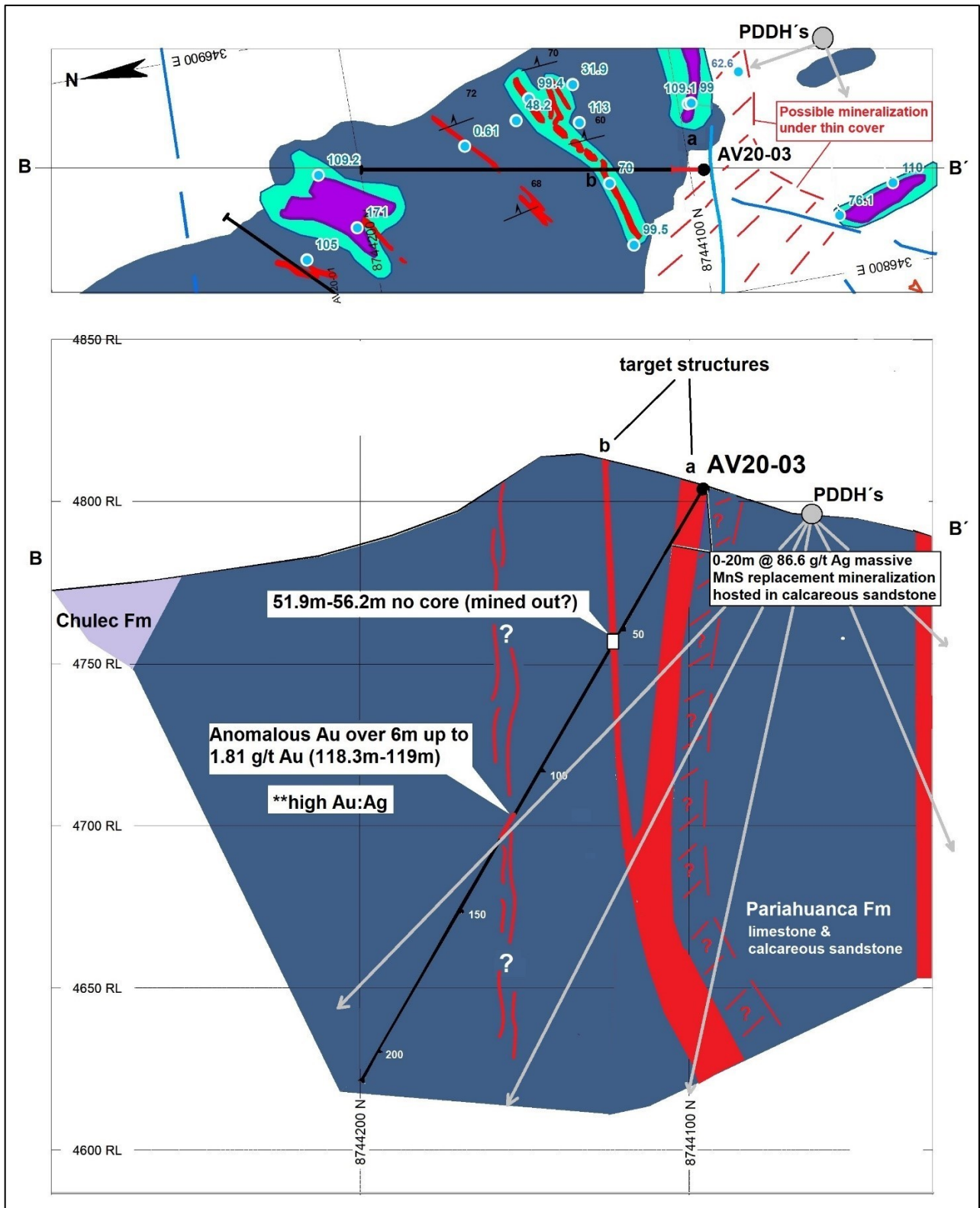
Figure 10.3 AV20-03 drill section with interpreted geology and proposed follow-up drill holes
