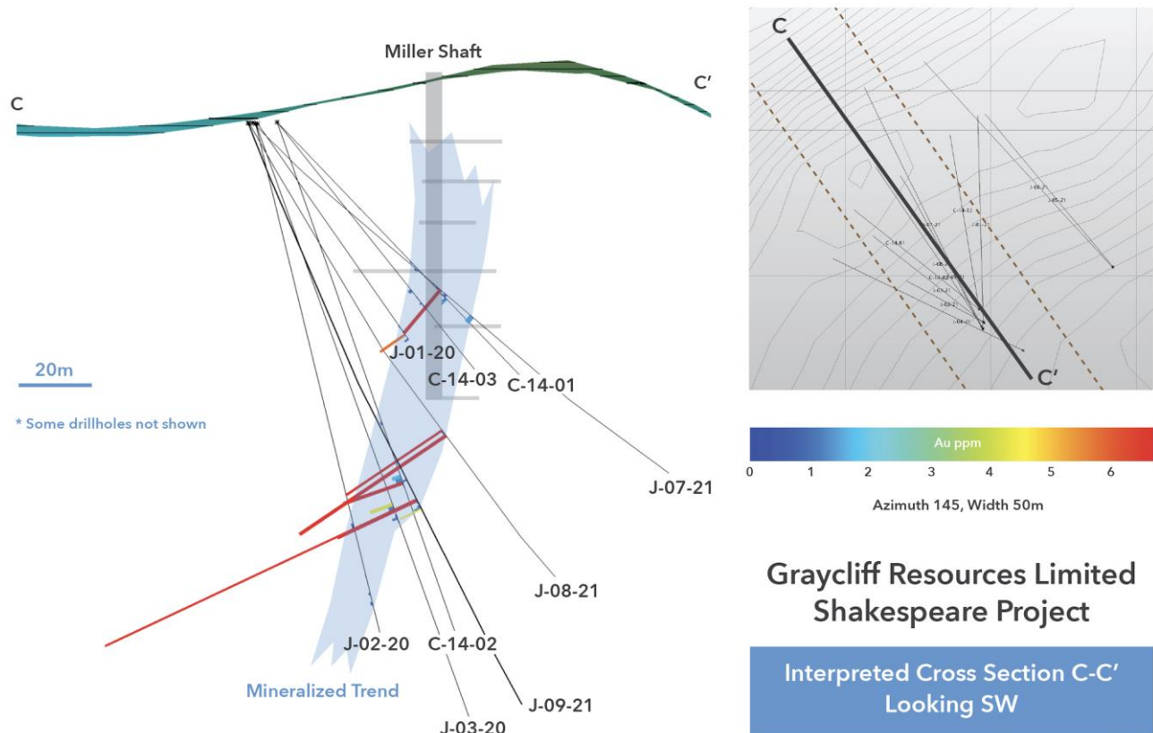
Figure 1 - Hole J-9-21 Location and Cross Section
