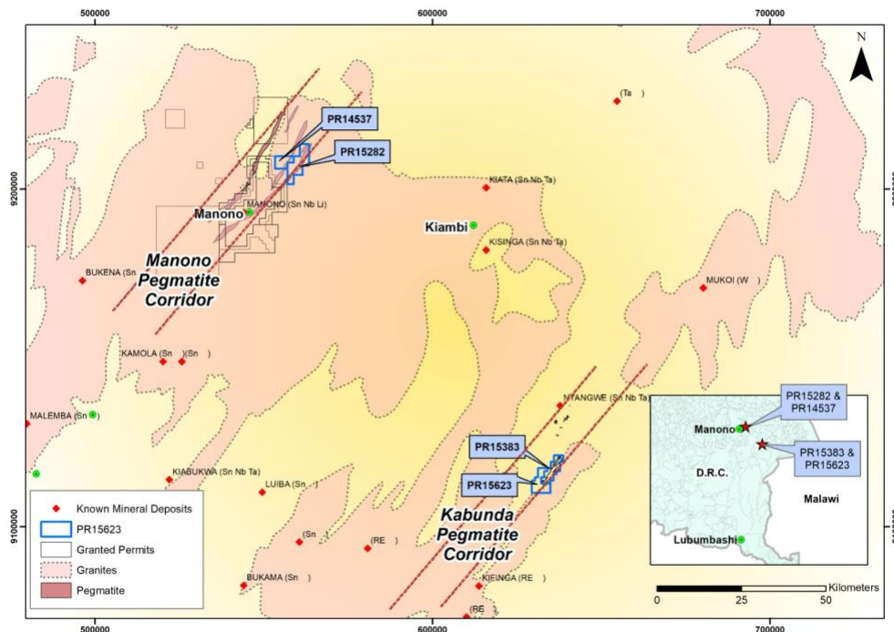
Figure 1: AJN Licences and the main Pegmatite Lithium Trends recognised in the Manono Region of Eastern DRC
