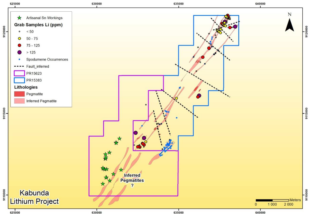
Figure 2: Permits PR 15623 and PR 15383 with Visible Spodumene Identified across both Licence Areas
