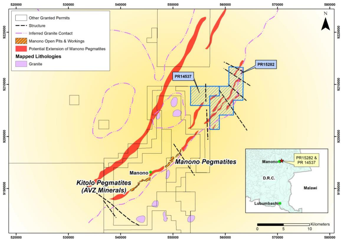
Figure 4: Potential Extension of Manono/Kitololo Pegmatites onto PRs 14537 and 15282
