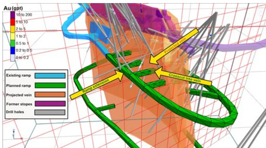
Mon Gold Mine Isometric View
