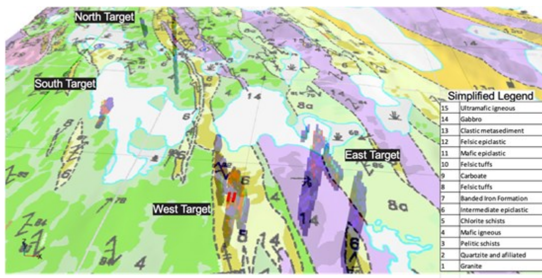
Figure 1. Isometric image of the four principal VMS targets looking north showing conductivity blocks on base map by Jackson V., (1998).
