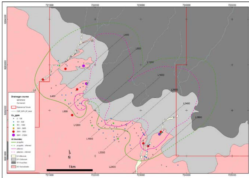
Figure 3. Simplified property geology map showing the distribution of the ~24 MaM Huaylillas pyroclastic sequence, unconsolidated colluvium derived from the pyroclastic sequence and the equigranular granodiorite host rock that is part of the Coastal Batholith. Mapped and inferred alteration boundaries shown in solid and dashed lines outline the target area. A propylitic alteration zone with dimensions 4.2 x 3.1 kilometre encloses potassic zone of 3.4 x 2.7 kilometre. Copper geochemistry from outcrop sampling is shown to highlight the relation of higher copper concentrations with mapped potassic alteration.
