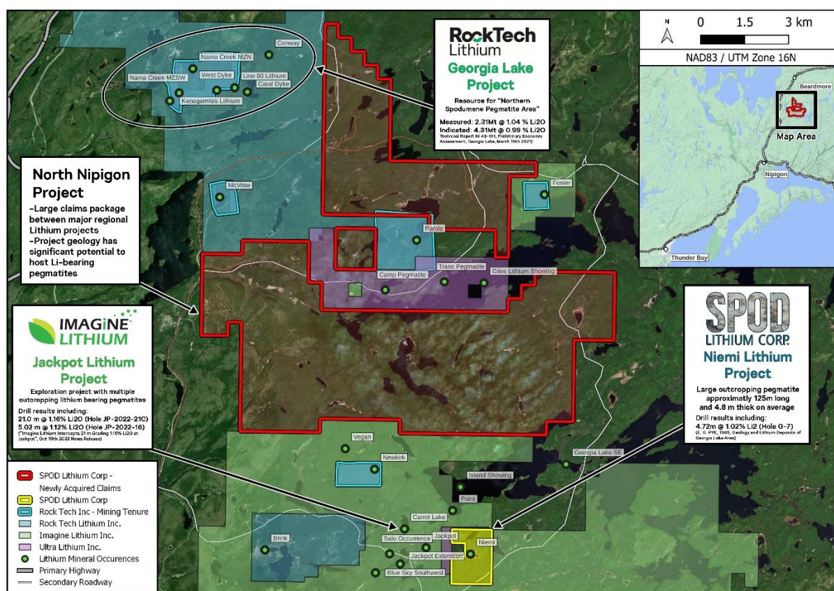
Figure 1: Map of the SPOD Lithium's existing and new mineral claims in the Georgia Lake area, with respect to other lithium explorers
