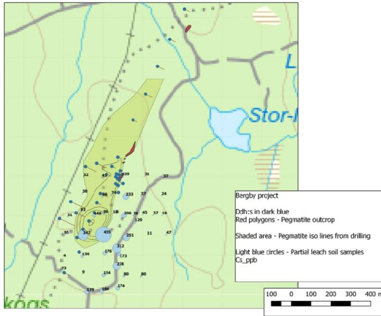
Figure 2 - Bergby lithium rich pegmatite and cesium soil samples
