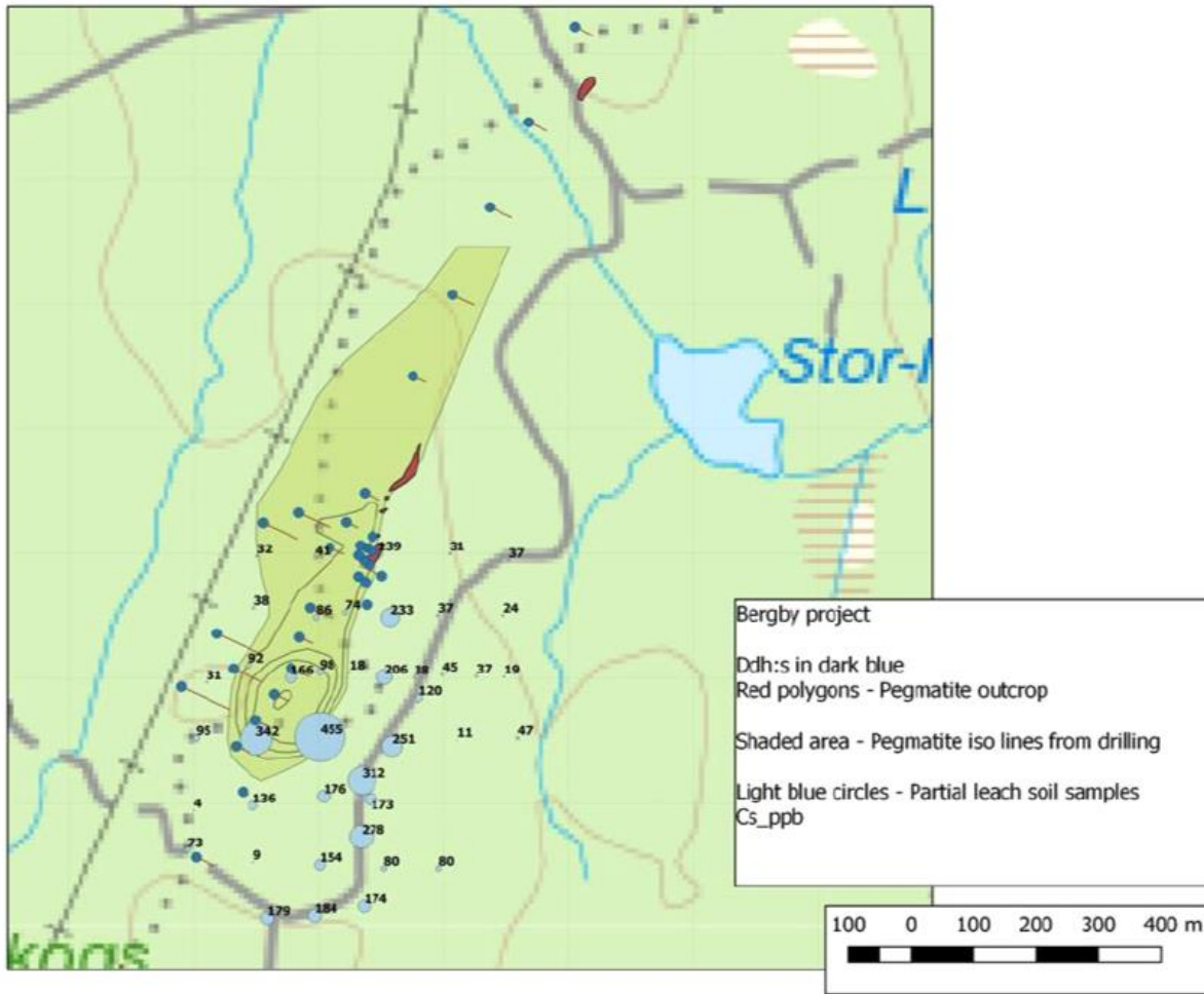
Figure 4 - Bergby lithium rich pegmatite and cesium soil samples
