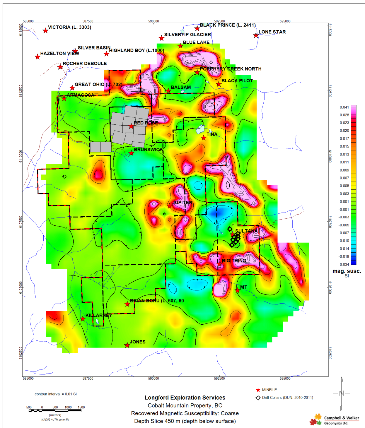
Figure 9.4 3d Voxi: 450m depth slice (below surface) through recovered susceptibility model (coarse).
