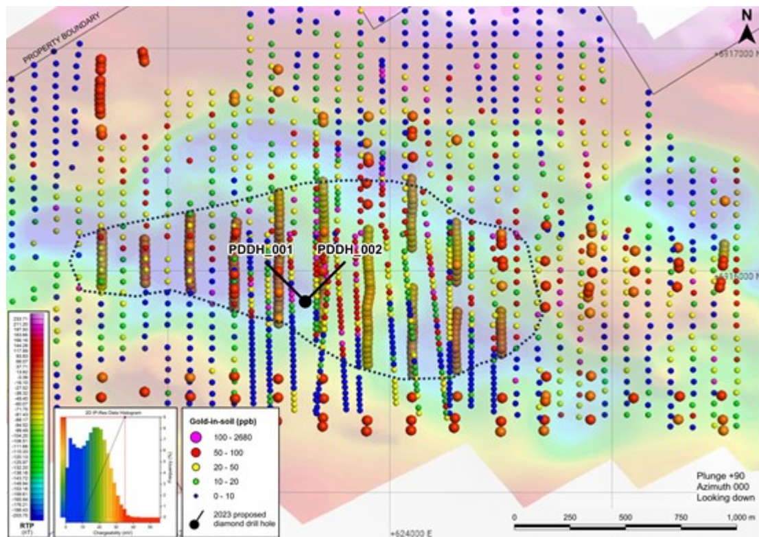
Figure # 2 shows the plan of chargeability results from the 2D IP-Res model overlain by gold-in-soil and magnetic susceptibility (RTP). The dashed polyline highlights the area of greatest interest for testing given the occurrence of favorable geochemical and geophysical anomalies. Also shown is the initially proposed 2 NQ diamond drill holes, each testing up to 500-meters in depth.
