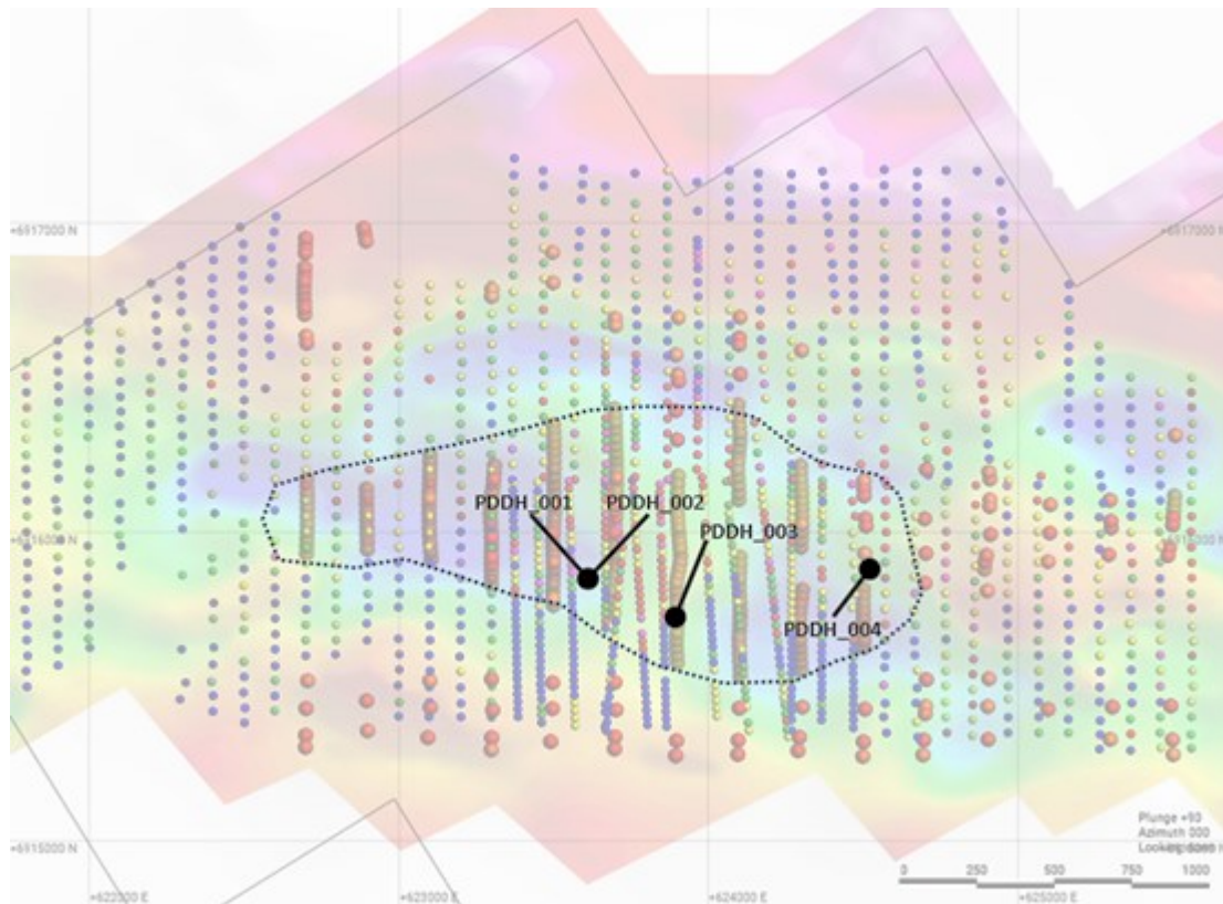
Figure 2. Proposed 4 NQ diamond drill holes, each testing to a 500-meter depth.
