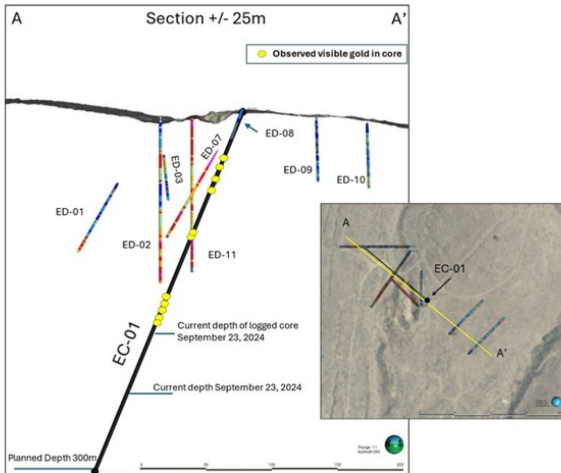
Figure 1 - Down dip visible gold locations in EC-01.
