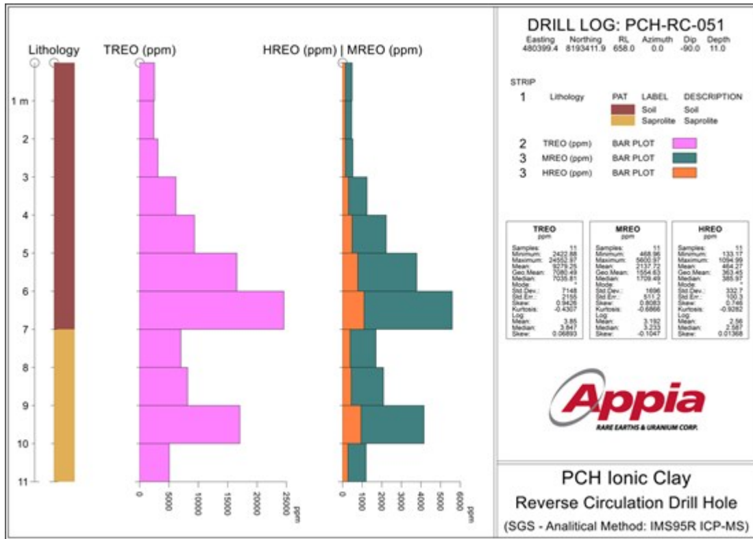
Chart #1 — PCH-RC-051 Drill Log
