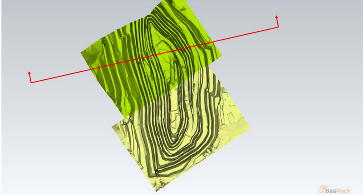
Figure 16-6: Bibiani Main Pit Central NW Slope Failure Back-Analysis Section
