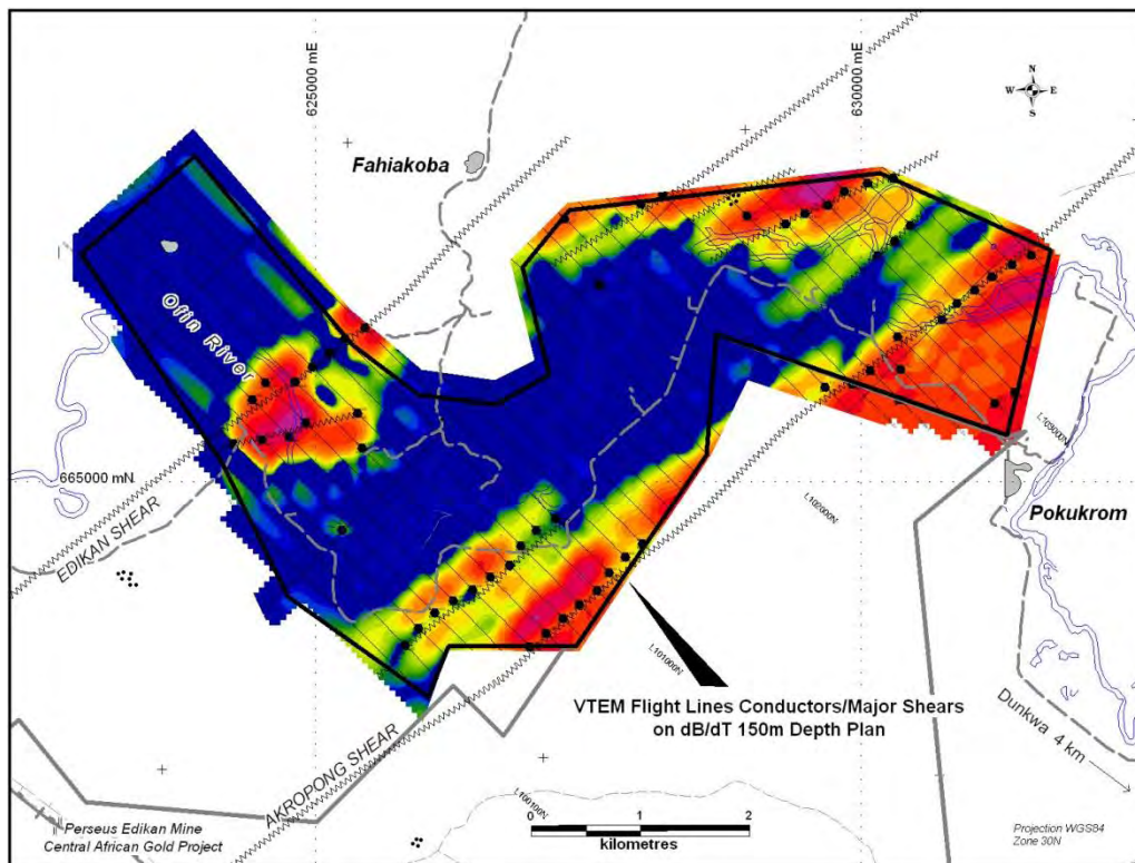
Figure 9.3.2 Geotech VTEM dB/dT Conductivity Depth Inversion Plan – 150m depth
