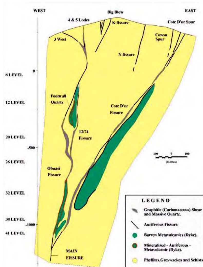
Figure 23.2.2 Section through the Fissure System around Kwesi Mensah Shaft area at Obuasi (Cox and Amanor, 1999).
