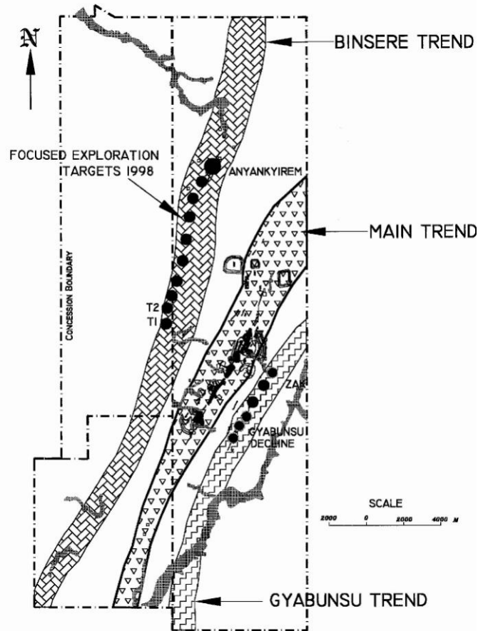
Figure 23.2.1 The Obuasi Concession showing the main mineralized corridors 1997 evaluated deposits, targets for 1998 onwards and prospects on the Gyabunsu Trend (Cox and Amanor, 1999).
