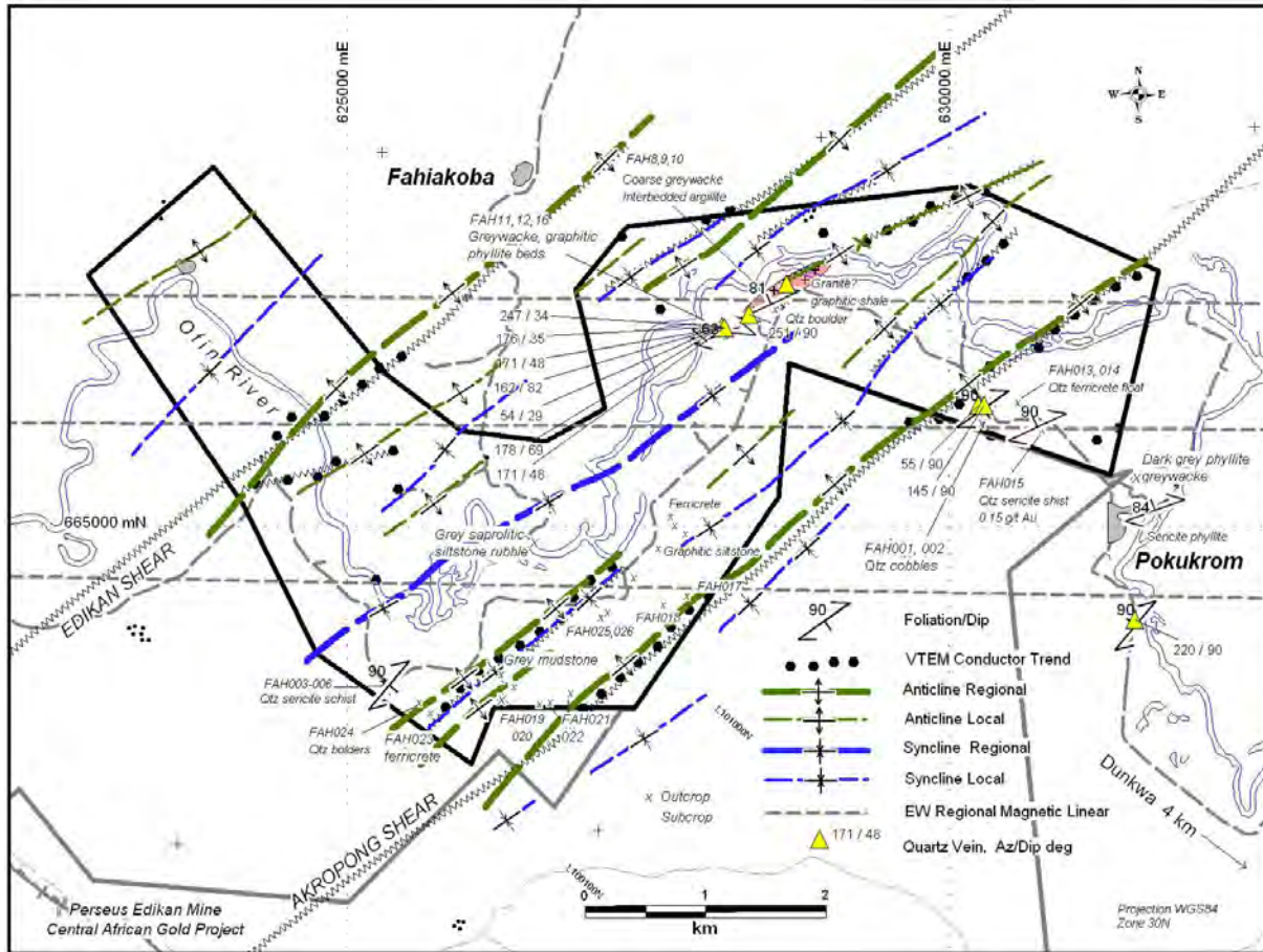
Figure 9.5.1 Geological mapping plotted on Geophysical-Geological interpretation.
