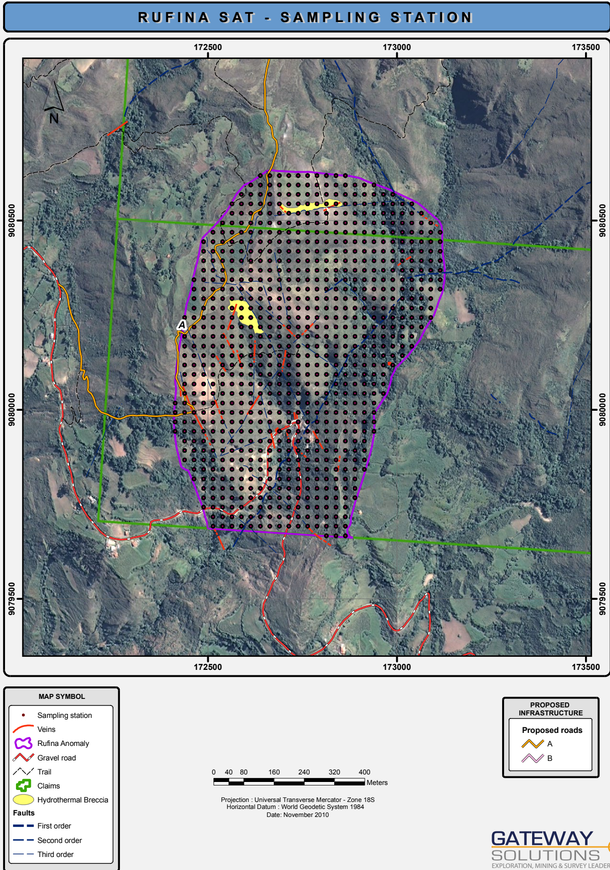
Figure 22.3. The proposed soil survey grid for the Rufina anomaly.
