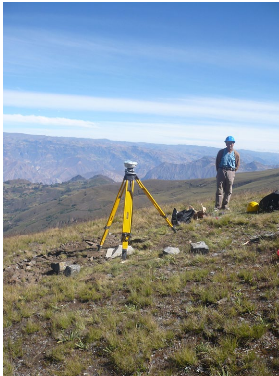
Figure 12.3. A GPS 5800 II measuring the A006 C-Order benchmark.
