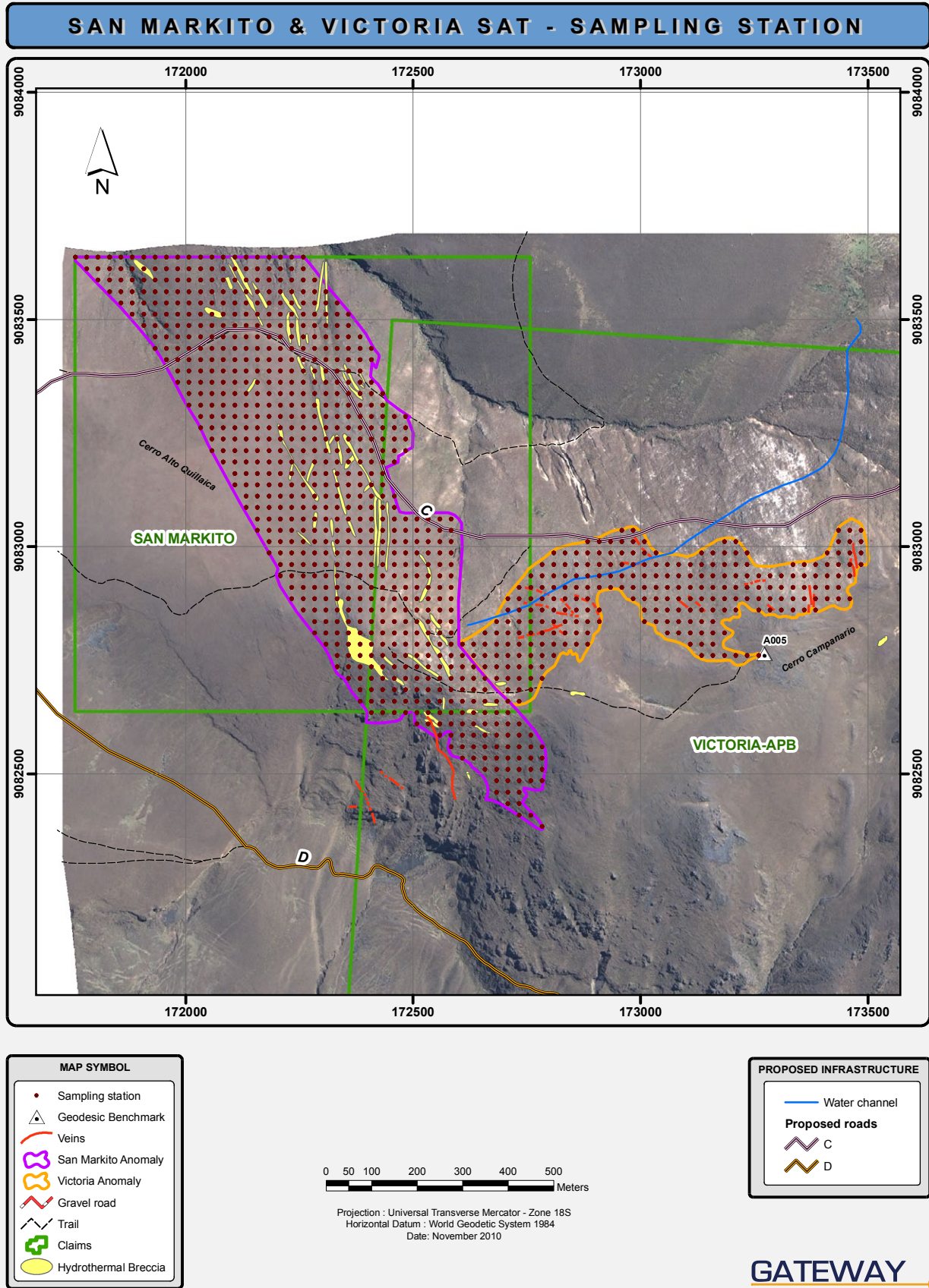
Figure 22.2. The proposed soil survey grid for the San Markito and Victoria anomalies
