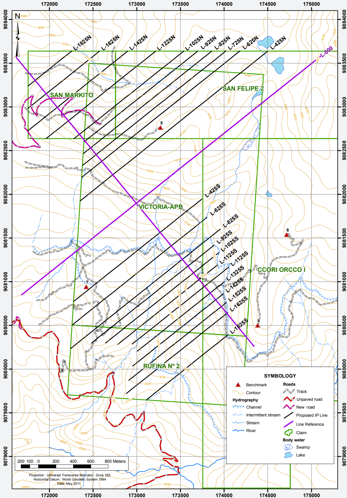
Figure 22.4. The proposed IP lines.
