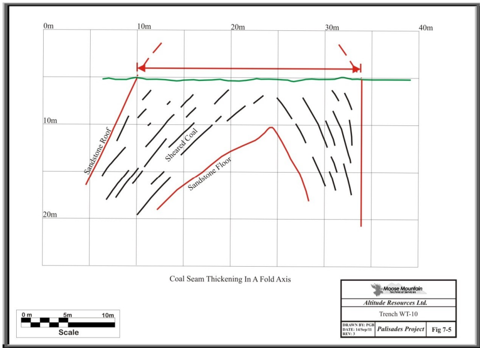
Figure 8. Trench WT-10
