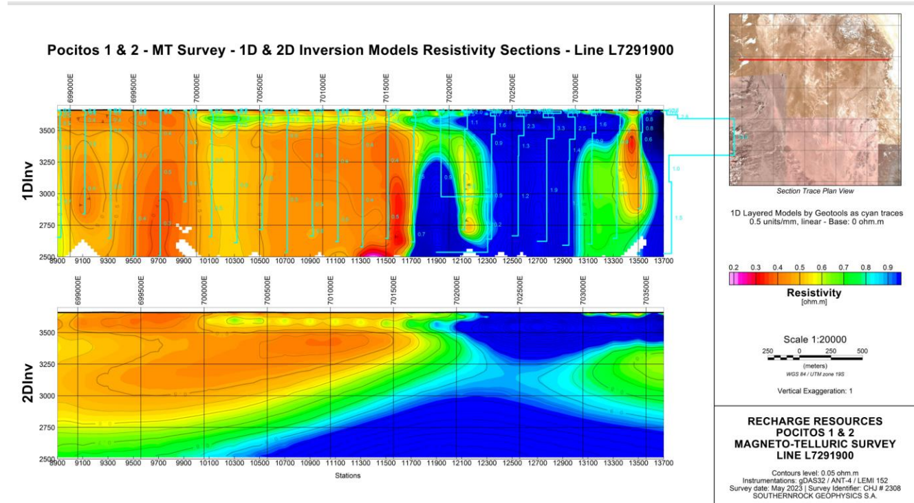
Figure 2. The 1D one dimensional point diagram shows highly conductive zones. Most notable is that the highest resistivity is only 0.9 Ohm-m, which is usually considered an excellent value for lithium containing brines. The 2D inversion (two dimensional section) shows a anticlinal structure in the centre and an ellipsoidal unit 2.5km long on the western part of the concession with evaporitic material on the surface and a paleo-channel in the top 250m.
