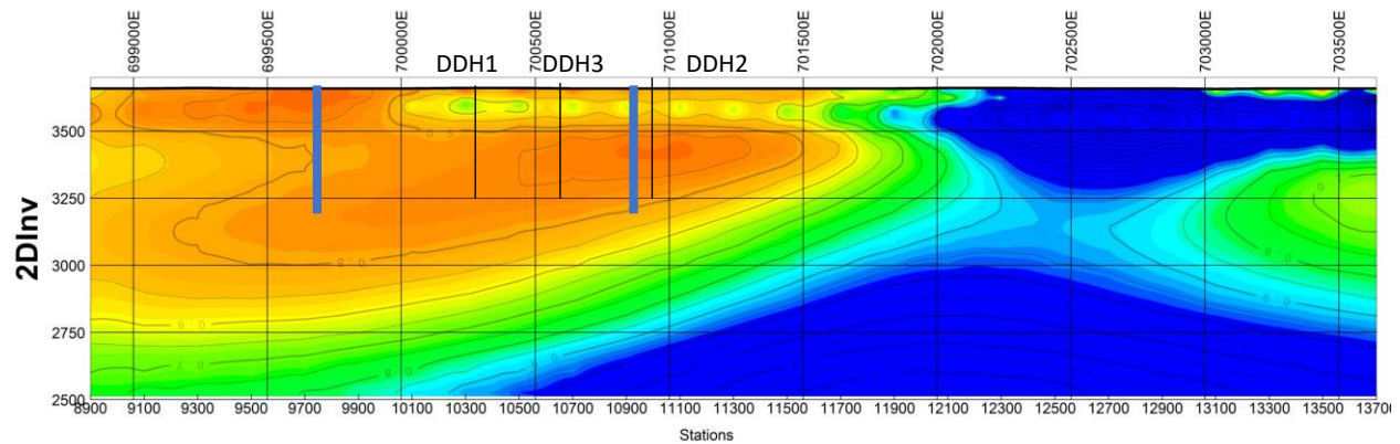
Figure 2. The 1D one dimensional point diagram shows highly conductive zones. Most notable is that the highest resistivity is only 0.9 Ohm-m, which is usually considered an excellent value for lithium containing brines. The 2D inversion (two dimensional section) shows a anticlinal structure in the centre and an ellipsoidal unit 2.5km long on the western part of the concession with evaporitic material on the surface and a paleo-channel in the top 250m.
