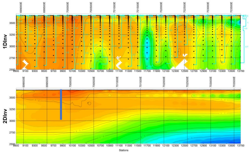
Figure 4. The southern most line shows an ellipsoidal body with resistivity below 0.5 Ohm-m extending for 4.5km. Blue line shows proposed exploration well. The total area of the Pocitos 1 is 800 Has and Pocitos 2 532 Has.
