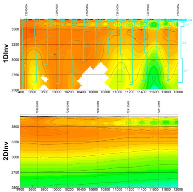
Figure 5 Line 1750 is north south on the boundary of Pocitos 1 and 2 and shows low resistivity in the northern section.
