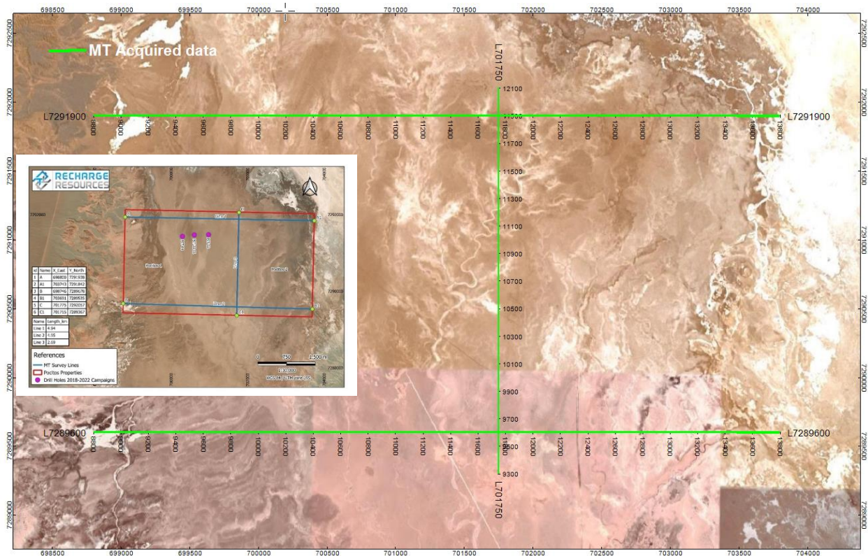
Figure 1. Map of the MT survey lines completed in early June 2023 WITH INSERT showing boundaries
