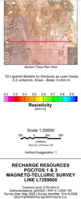
Figure 4. The southern most line shows an ellipsoidal body with resistivity below 0.5 Ohm-m extending for 4.5km. Blue line shows proposed exploration well. The total area of the Pocitos 1 is 800 Has and Pocitos 2 532 Has.
