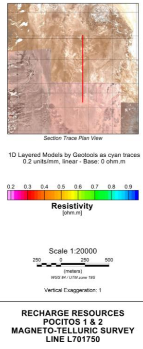
Figure 5 Line 1750 is north south on the boundary of Pocitos 1 and 2 and shows low resistivity in the northern section.
