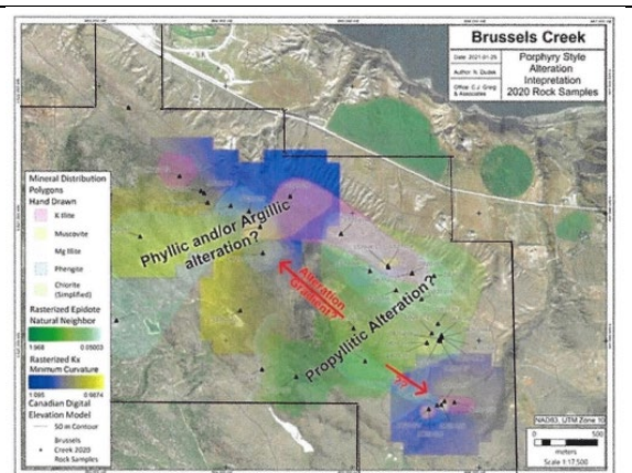
Figure 2. Porphyry-style Alteration Interpretation from Hyperspectral Study
