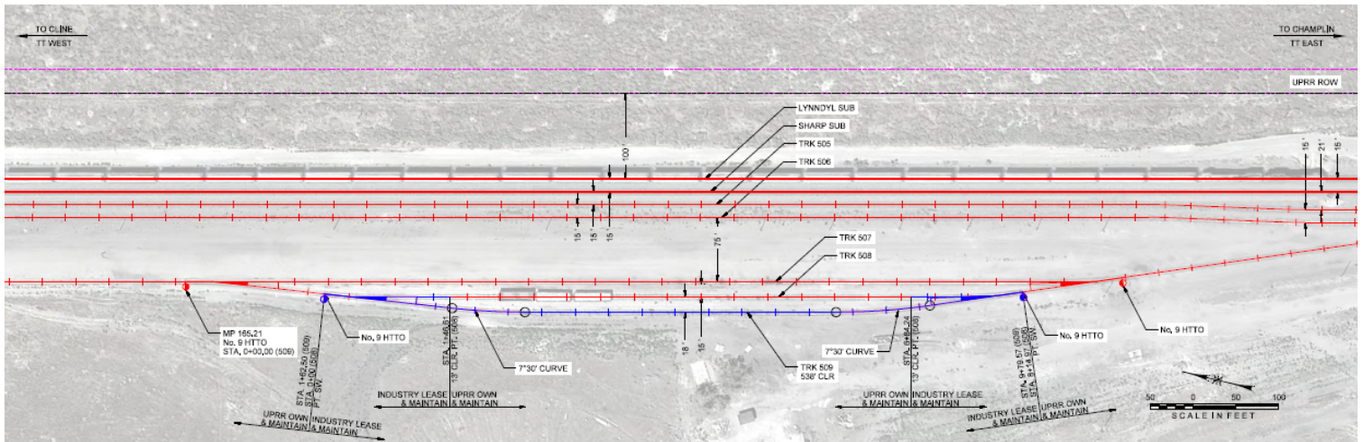
Rail Spur Schematic Layout
