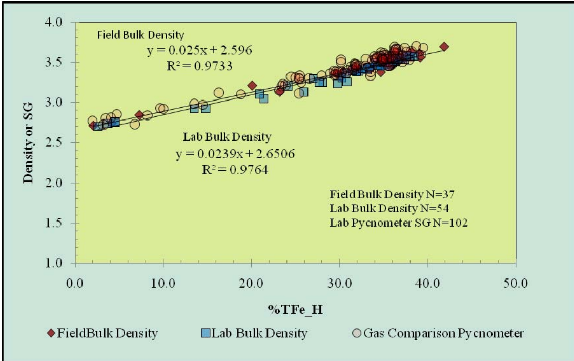
Figure 14. In-field bulk density
