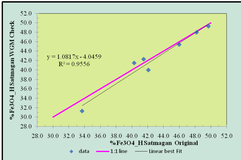
Figure 23. %Fe 3 O 4 _H Satmagan for WGM Check vs. Raytec Original
