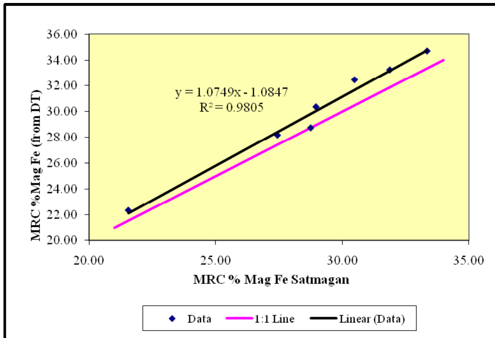
Figure 27. %Magnetic Fe from Davis Tube at MRC vs. Satmagan Method at MRC
