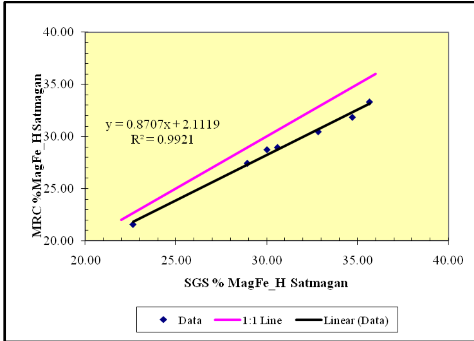
Figure 26. %Magnetic Fe by Satmagan method for MRC vs. SGS-Lakefield
