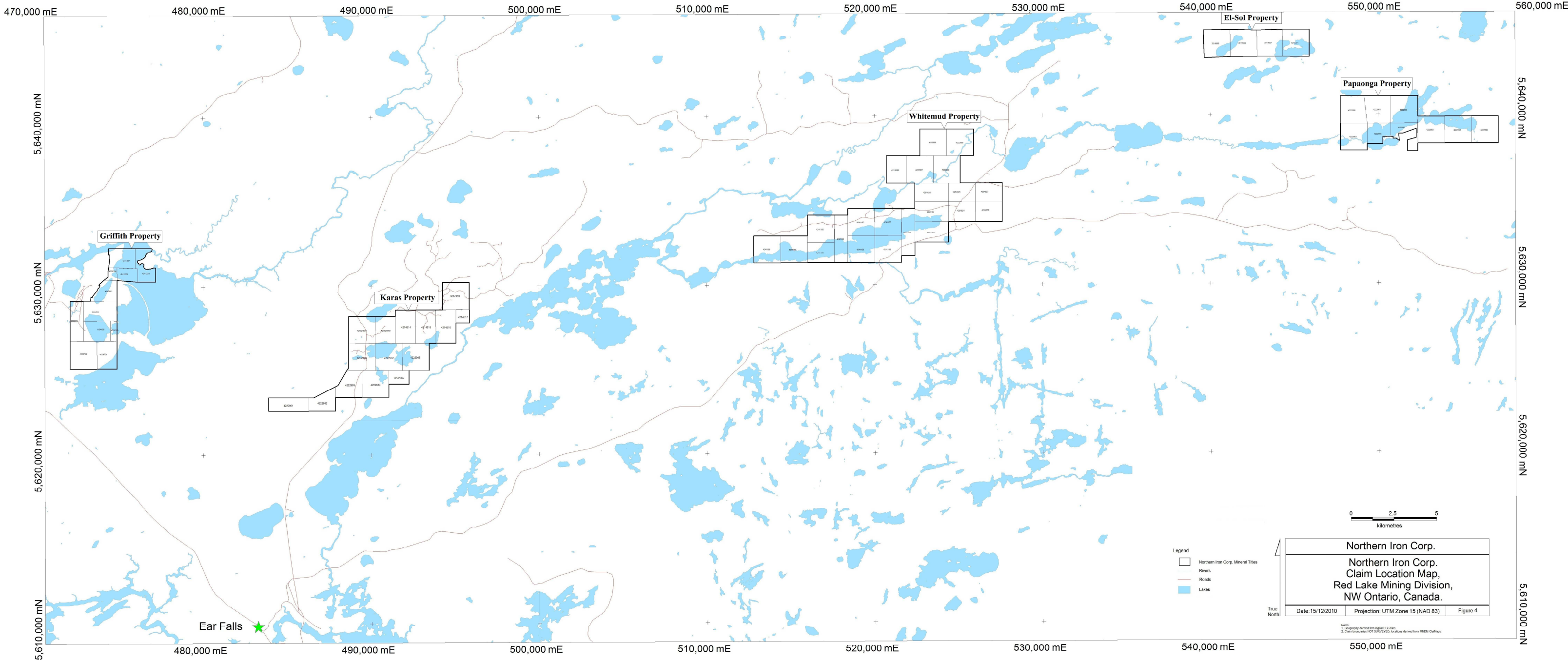
Figure 4: Northern Iron Corp. Property Locations, Red Lake District, Ontario
