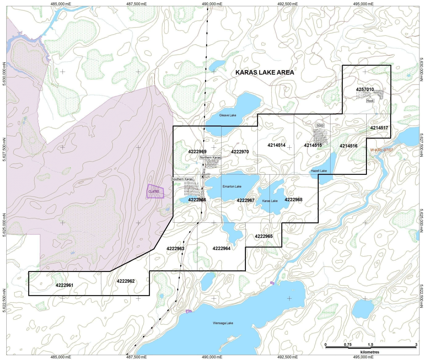
Figure 2: Karas Property Claim Location
