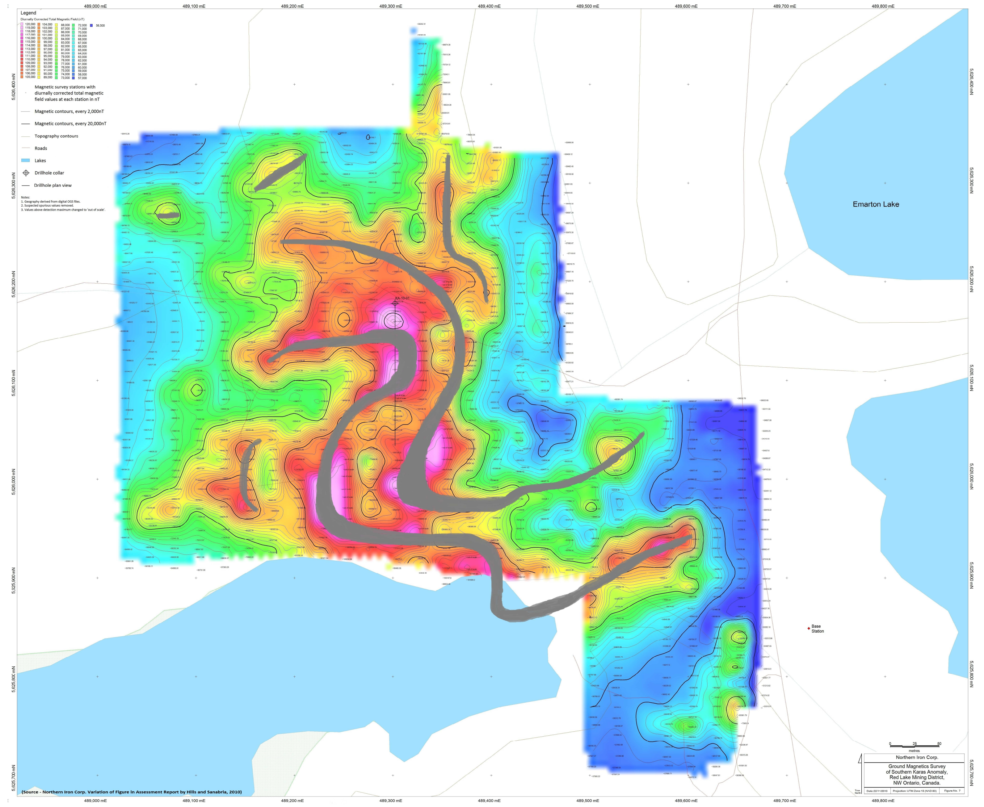
Figure 7: Karas South Magnetic Anomaly – BIF Superimposed
