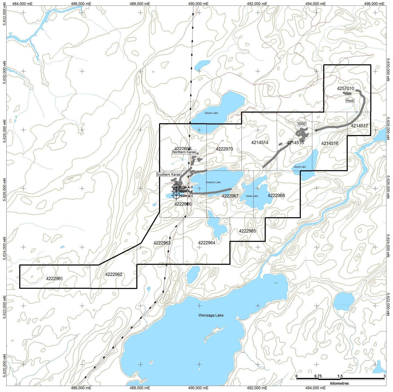
Figure 3: Karas Property Historical Deposit and Drill Collar Locations
