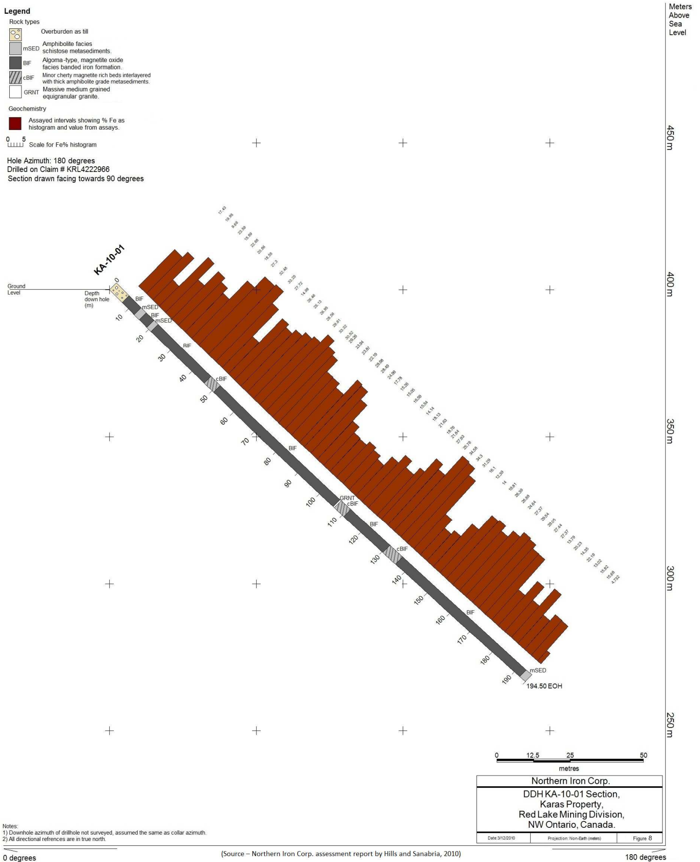
Figure 8: Karas South Occurrence DDH No. KA-10-01 Section
