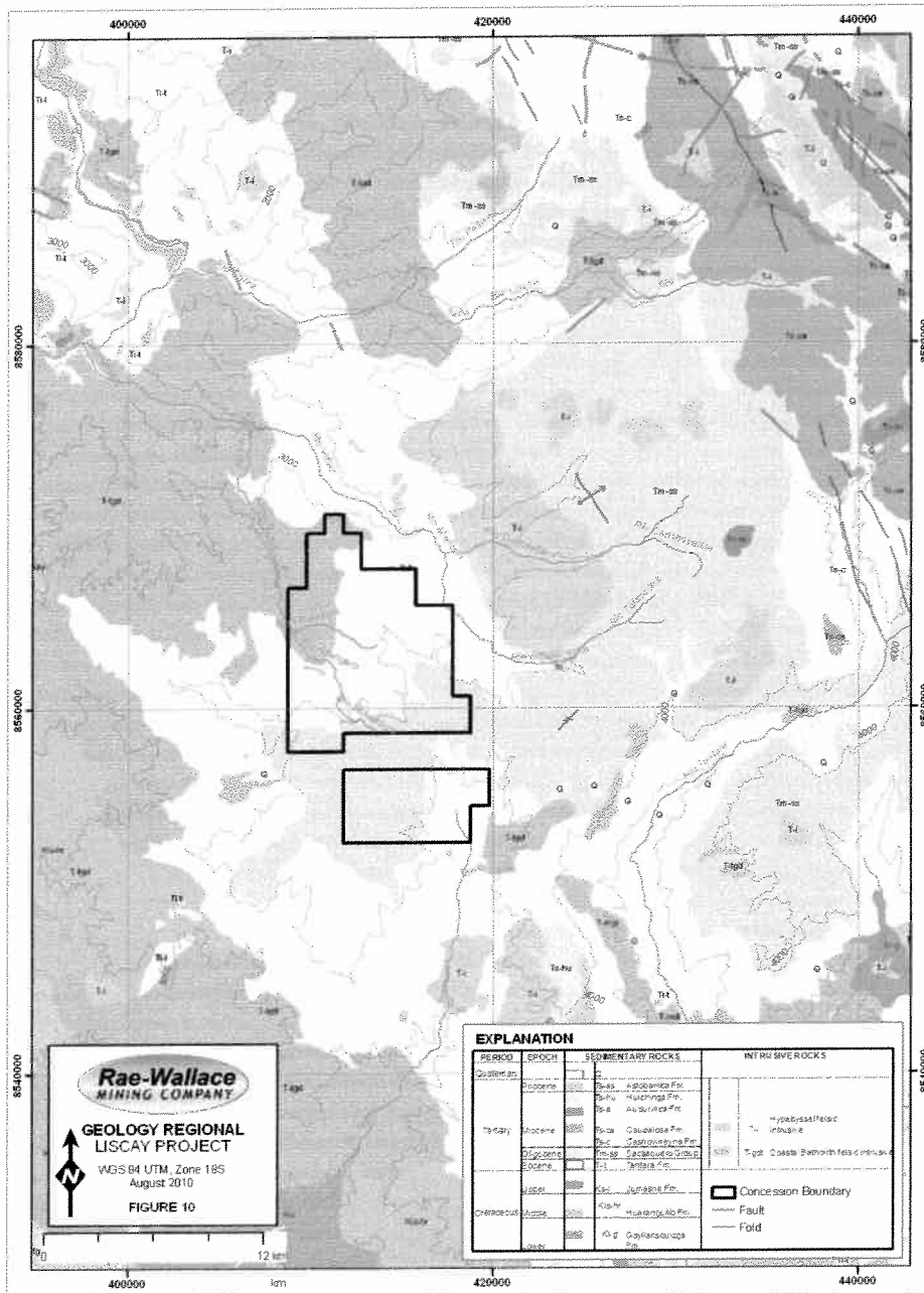
FIGURE 9-1: Liscay Regional Geology (from GIX files)
