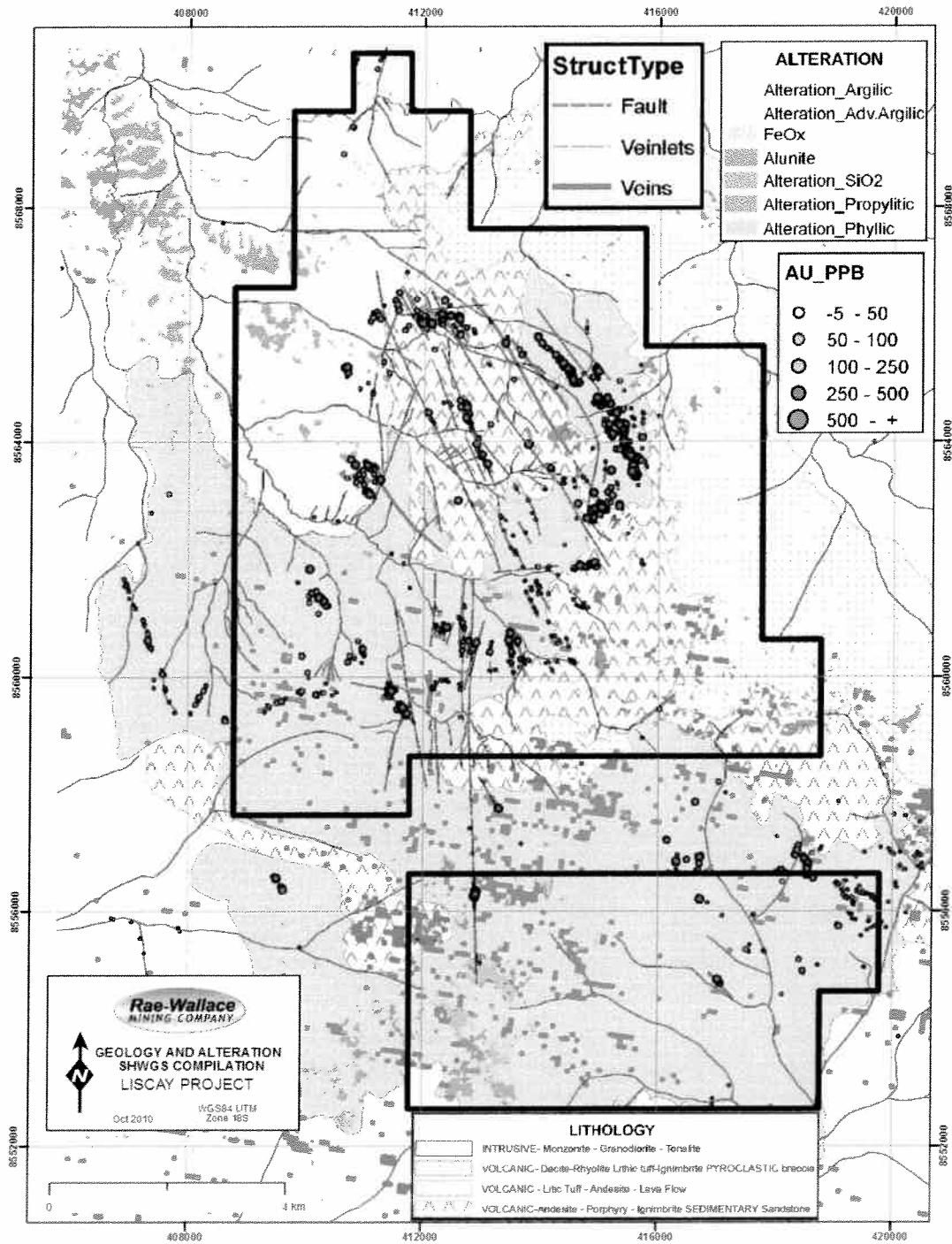
Figure 9-2: Geology, Structure and Alteration (from GIX files)
