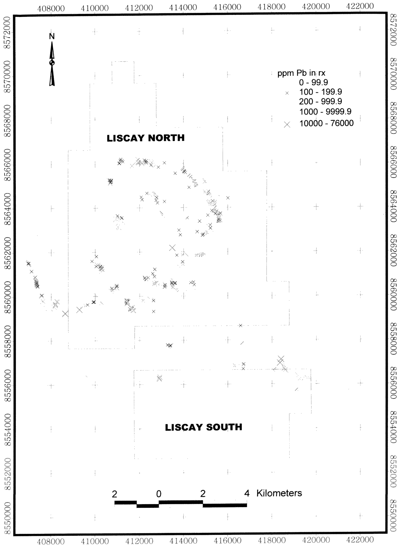
FIGURE 12-1C: LEAD IN ROCKS
