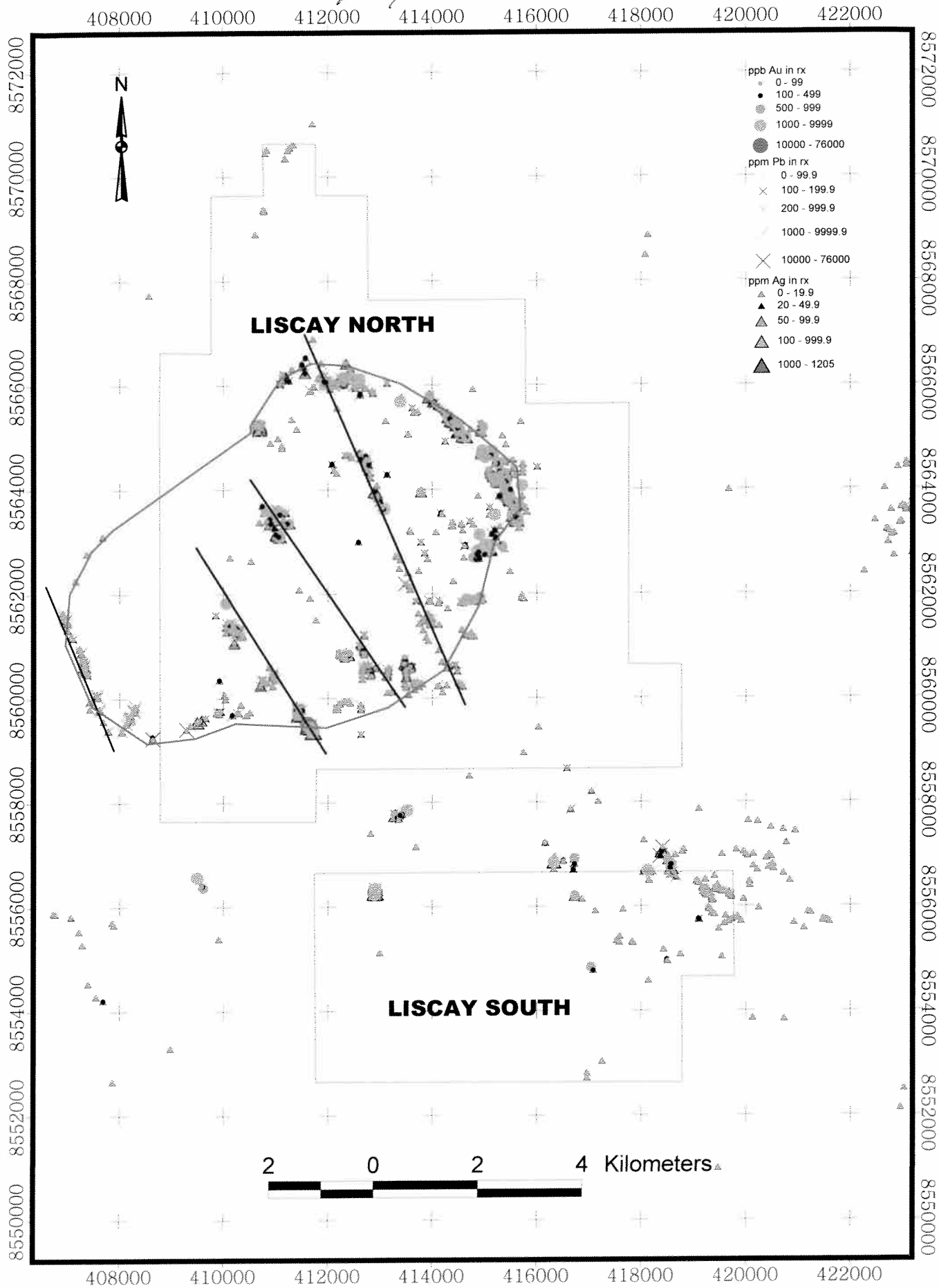
FIGURE 12-1D: ROCK GEOCHEMICAL COMPILATION SHOWING NOTIONAL CALDERA AND LINEAR ELEMENTS
