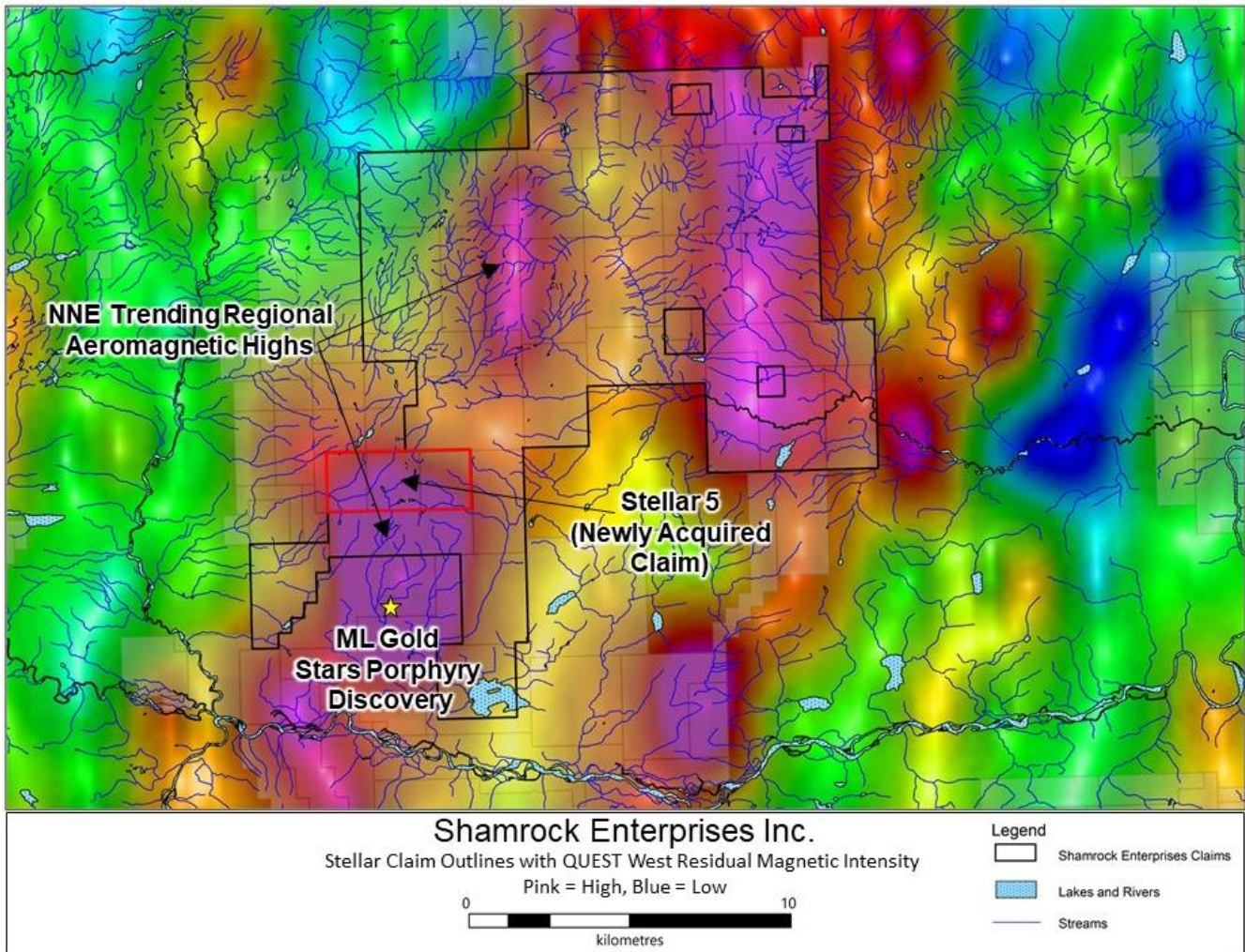
Figure 1: Shamrock's Newly Acquired Claim, NNE Trending Regional Aeromagnetic Highs and ML Golds Stars Discovery
