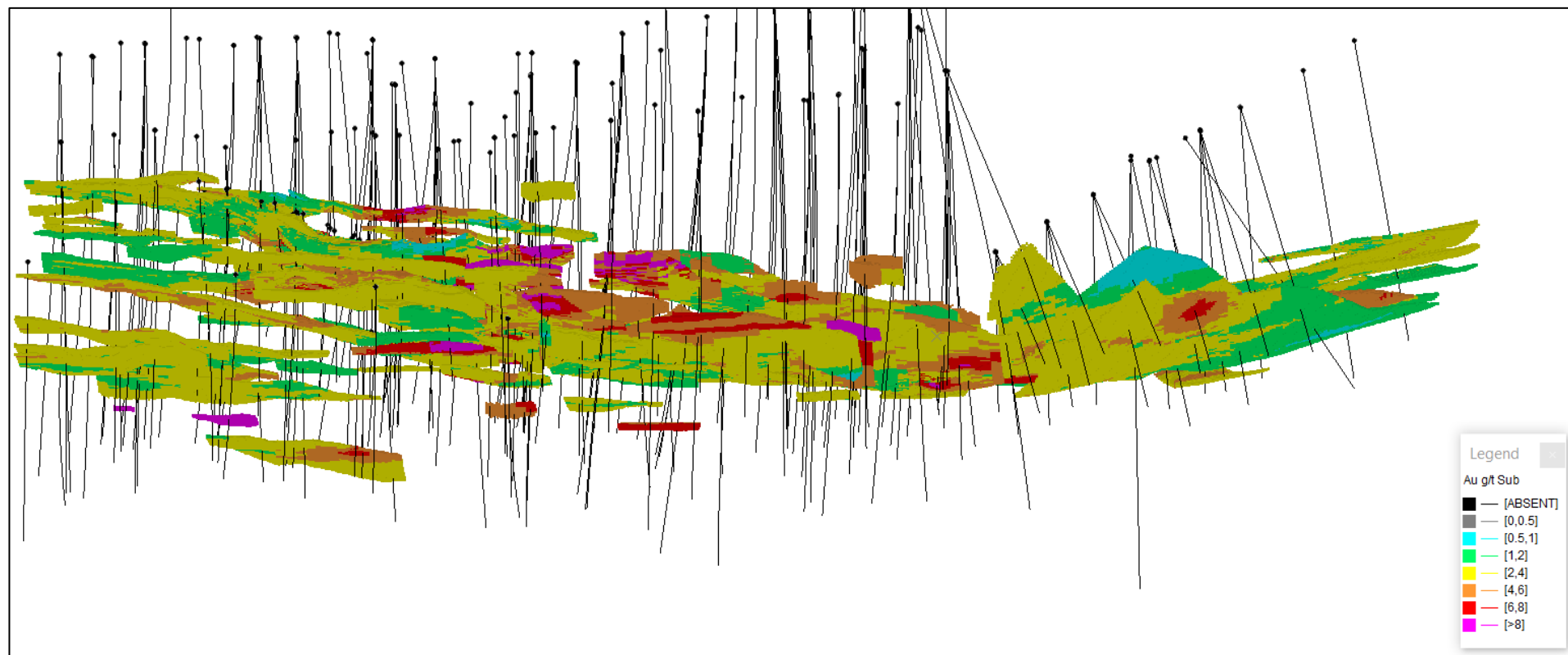
Figure 14-24: Perspective view, looking South of Block Model showing estimated grade (Au g/t) distribution in the mineralized lodes
