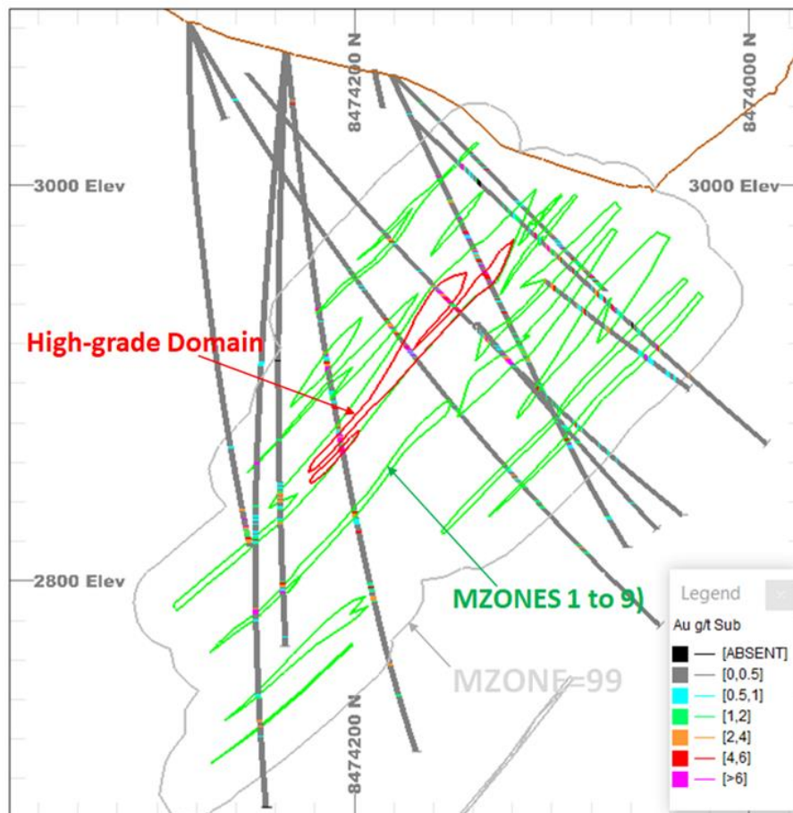
Figure 14-4: 2014 model - Cross-section 339,200 mE showing low-grade host rock domain (MZONE 99) modelled around mineralized lodes
