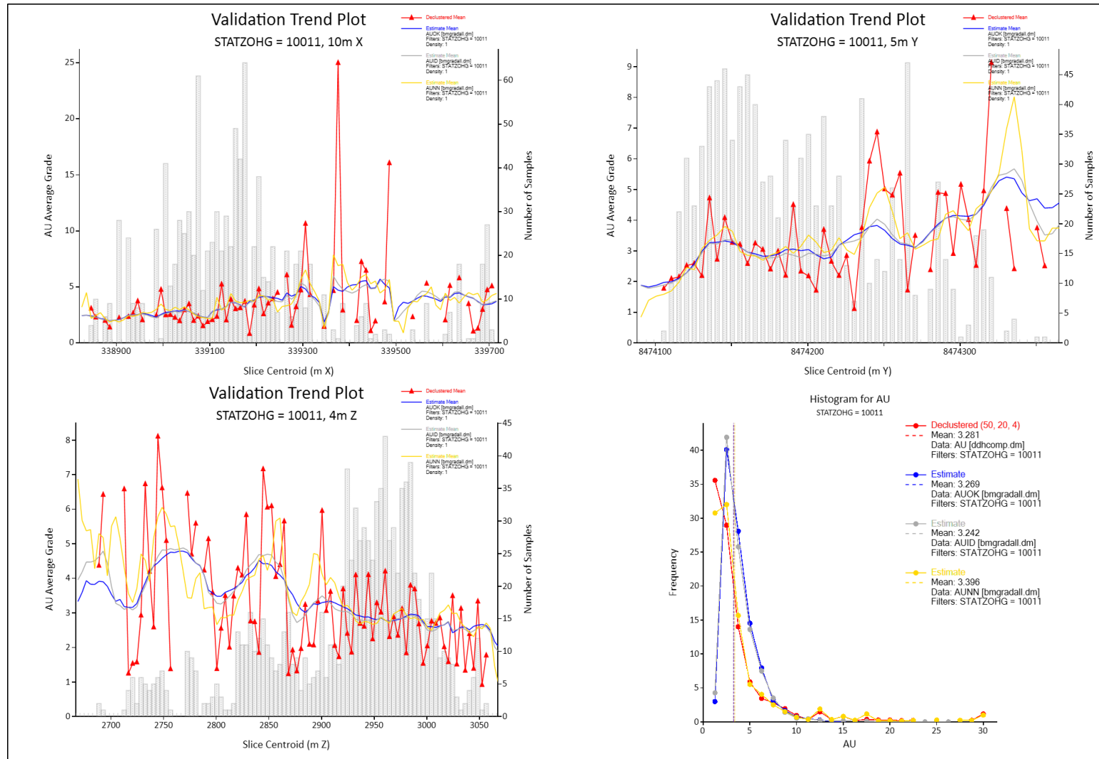
Figure 14-18: Comparison of model OK grade against composite sample declustered and model NN, on sections in the three axis: North, East and RL; (MZONE=1-Low grade)
