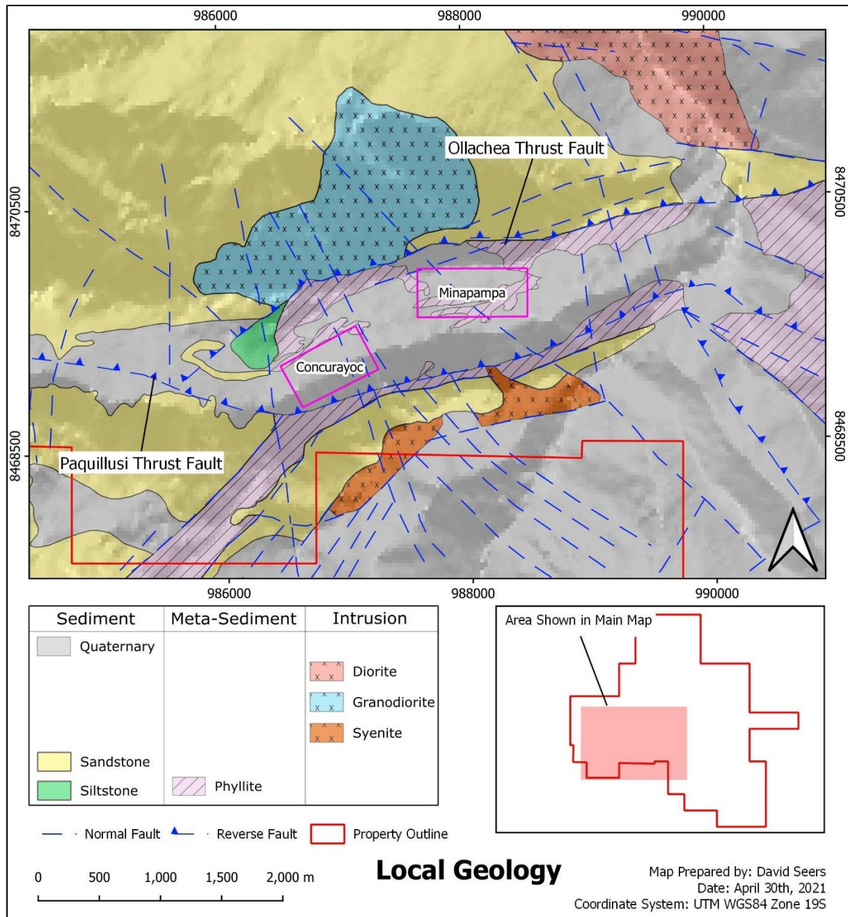
Figure 7-3: Property Geology
