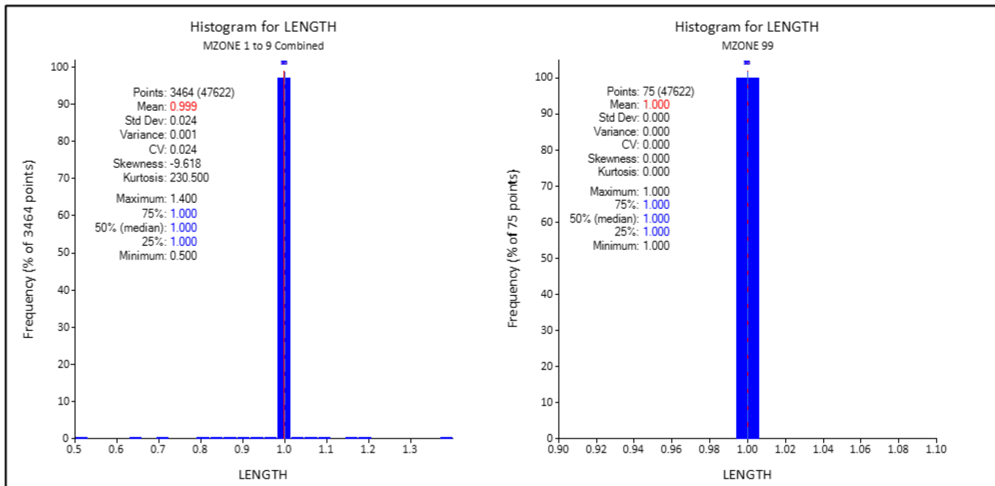
Figure 14-6: 1 m Composite Data - Sample intervals within Mineralized Lodes (left) and Host rock (right).
