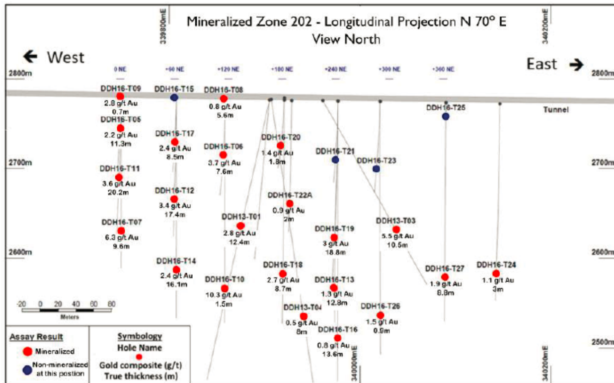
Figure 15 Longitudinal Projection of mineralized Zone 202 showing composite gold grade (g/t) and true thickness (m)
