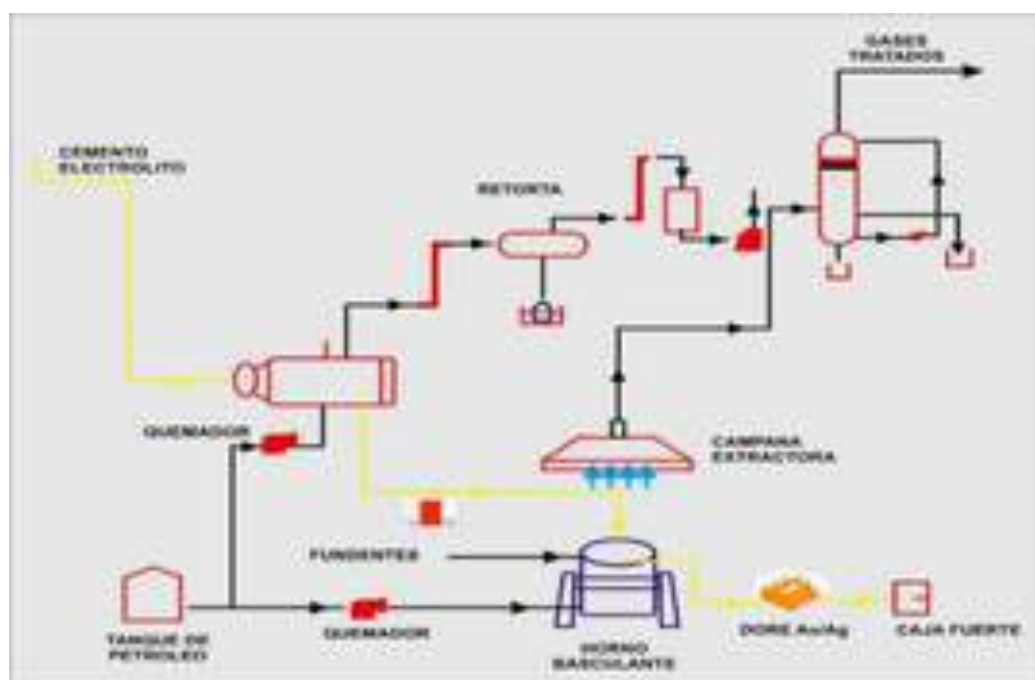
Figure 13.2.2-2: Harvesting and smelting process
