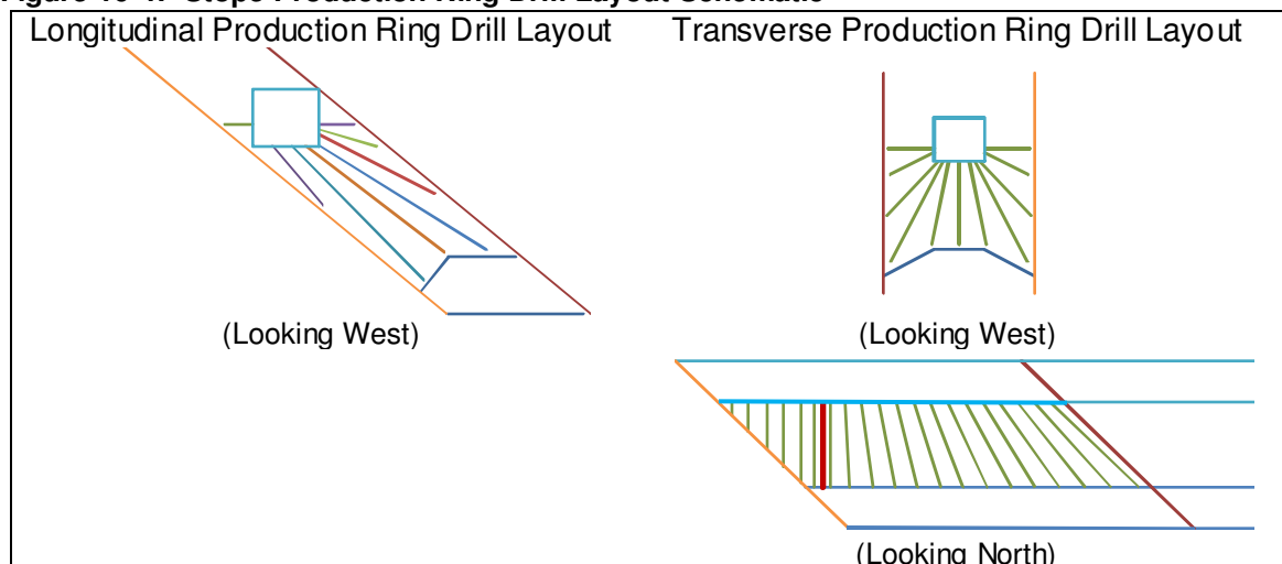
Figure 16-4: Stope Production Ring Drill Layout Schematic
