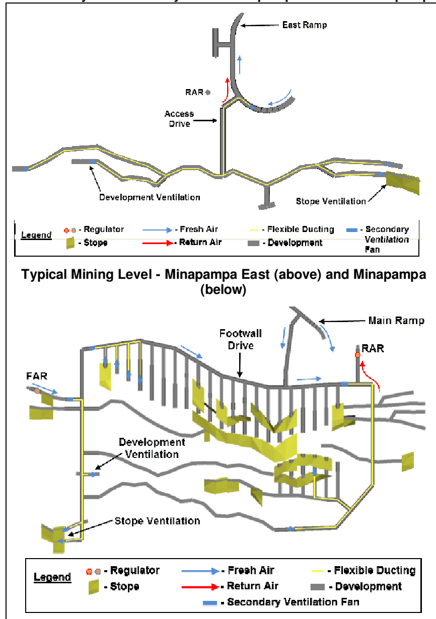
Figure 16-7: Secondary Ventilation System – Minapampa East and Minapampa
