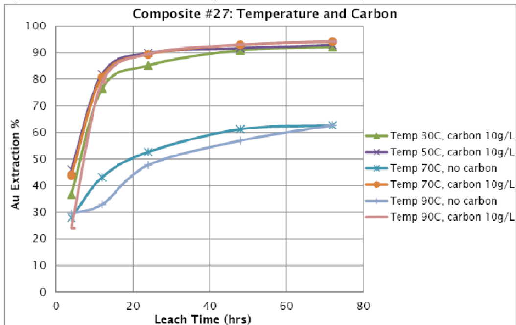
Figure 13-3: Effects of Leach Temperature and Carbon Population
