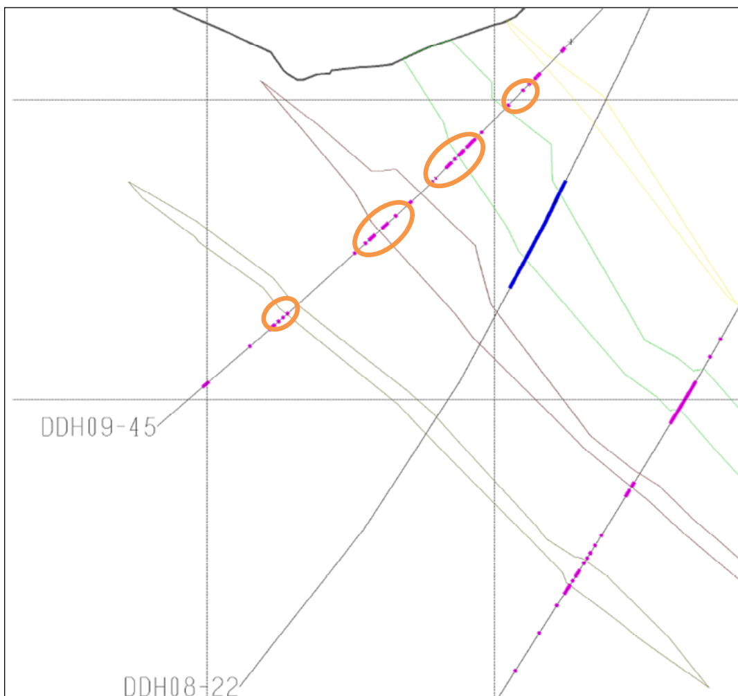
Figure 11-2: DDH09-45 Intervals and Lens Associations
