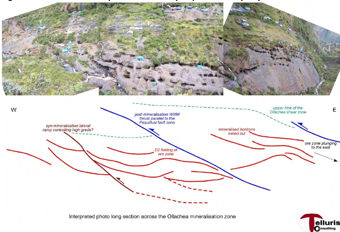
Figure 7-3: Structural Interpretation of Minapampa and Minapampa East Zones
