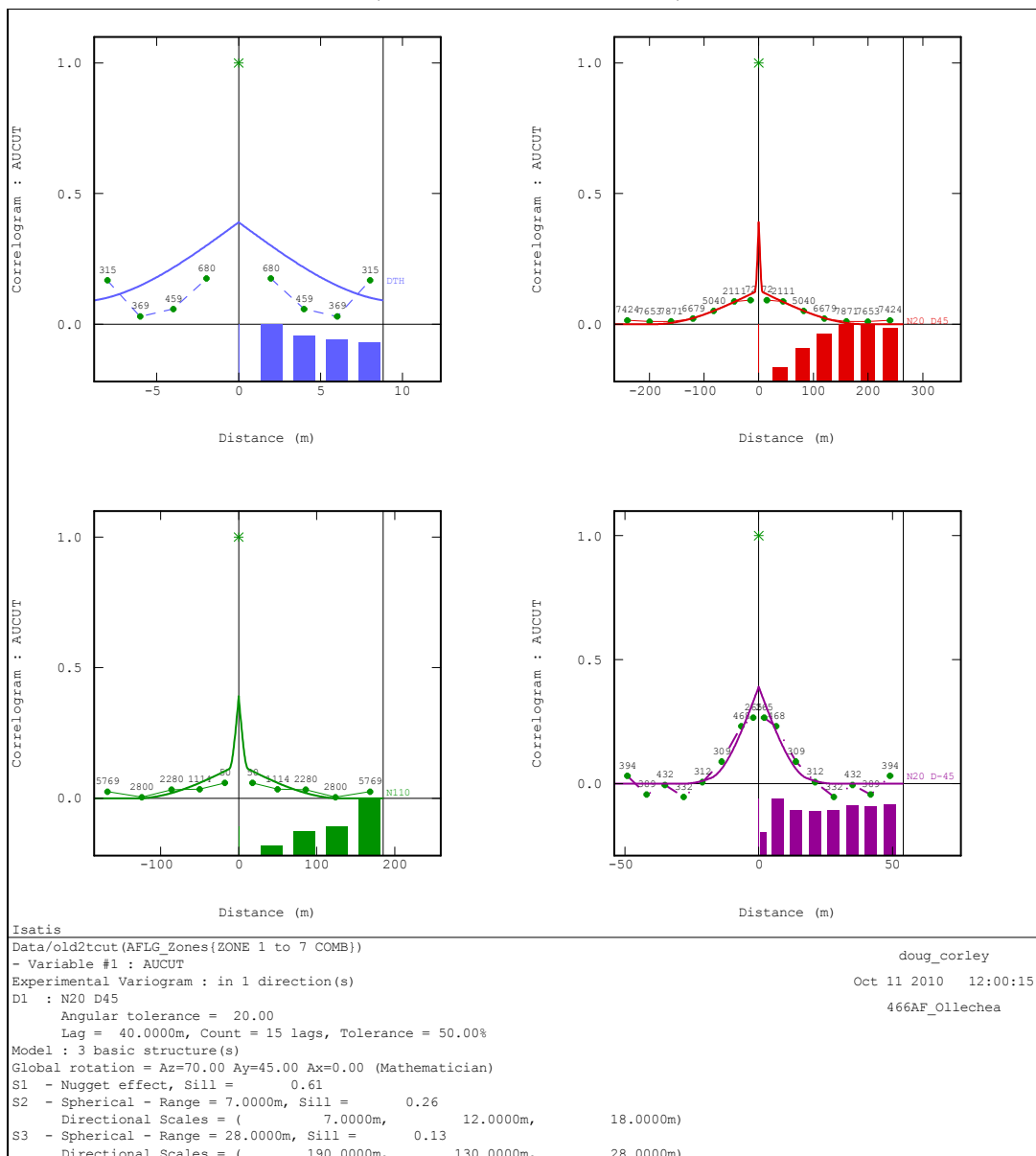
Figure 40 Ollachea Project Correlogram MINZONE=1 (Combined Mineralised Zones)
