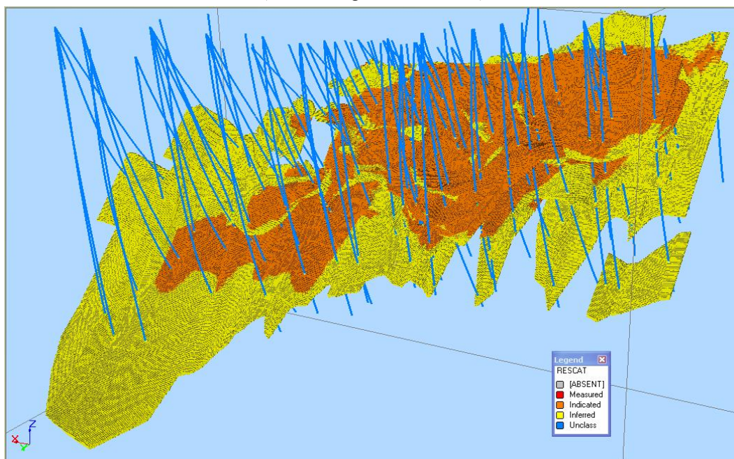
Figure 46 Ollachea Project : 3D Perspective View of Drilling Data and Inferred / Indicated Classified Blocks (view looking to the south-east)
