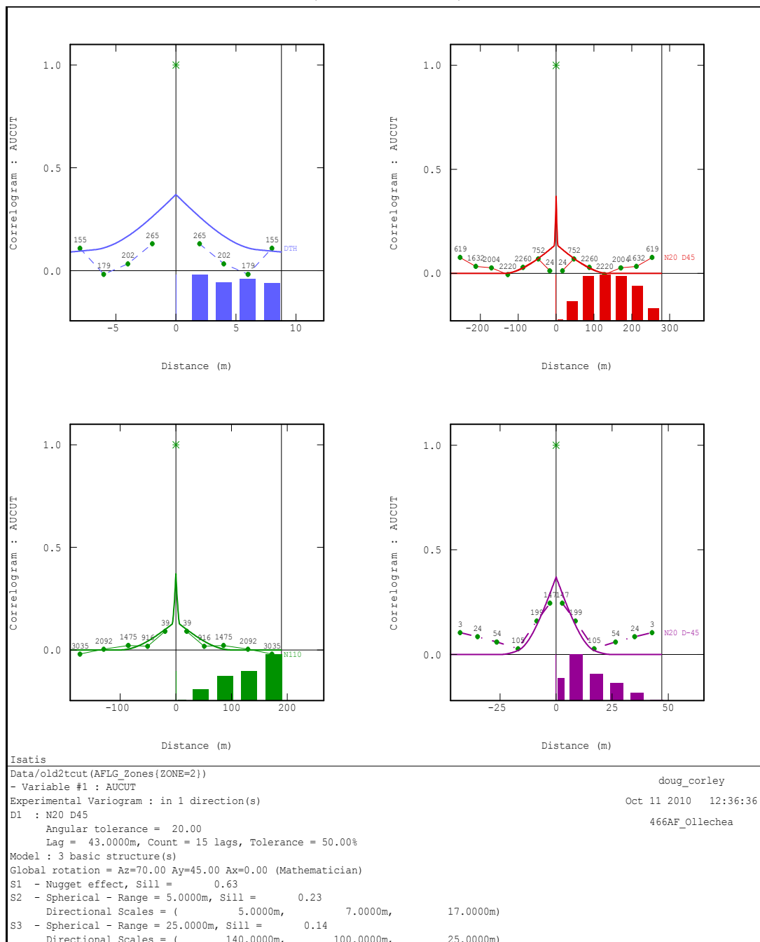
Figure 41 Ollachea Project Correlogram ZONE=2 (Mineralised Zone 2)
