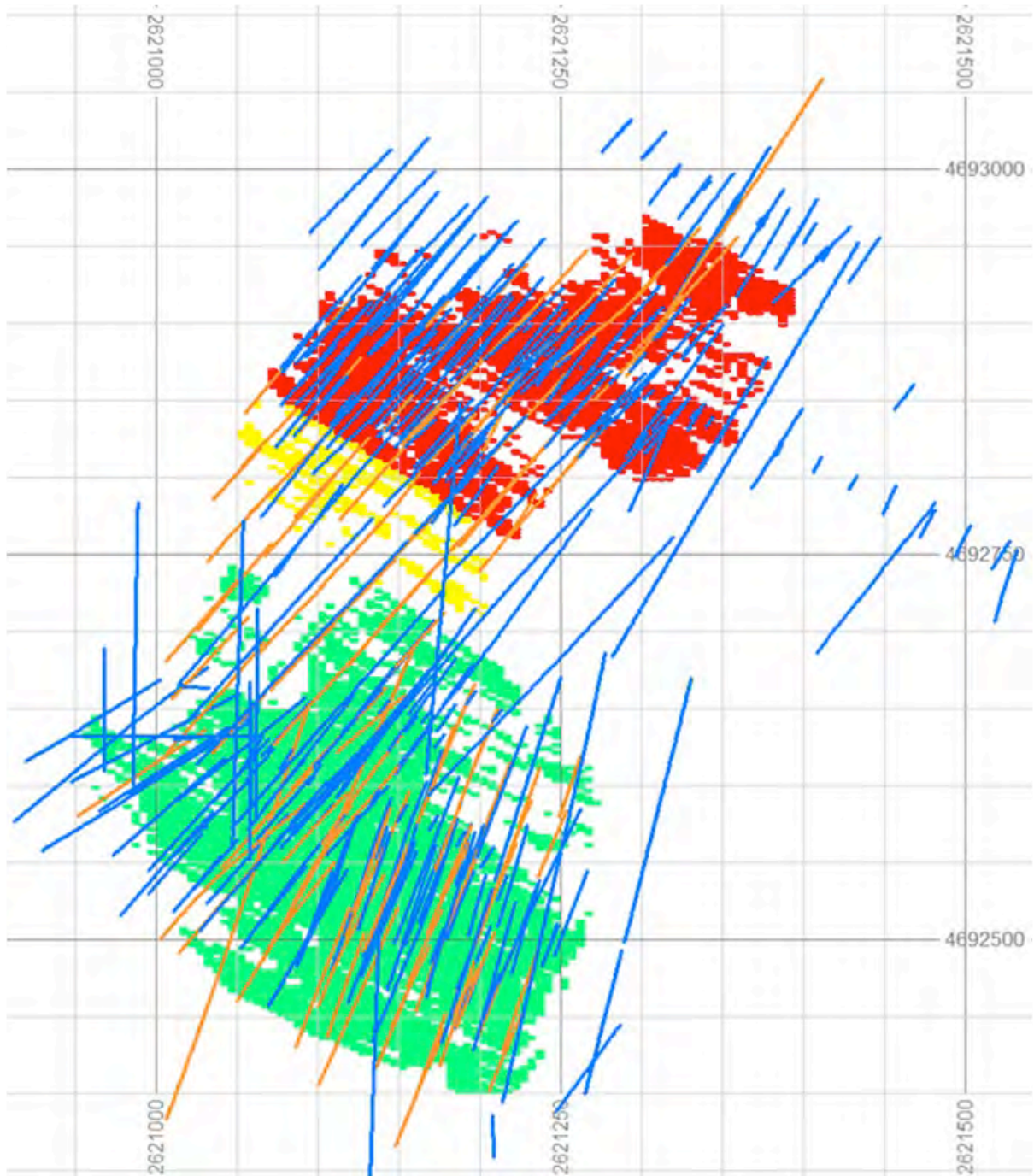
Figure 40 Martinetas Central Area Drill and Trench Plan
