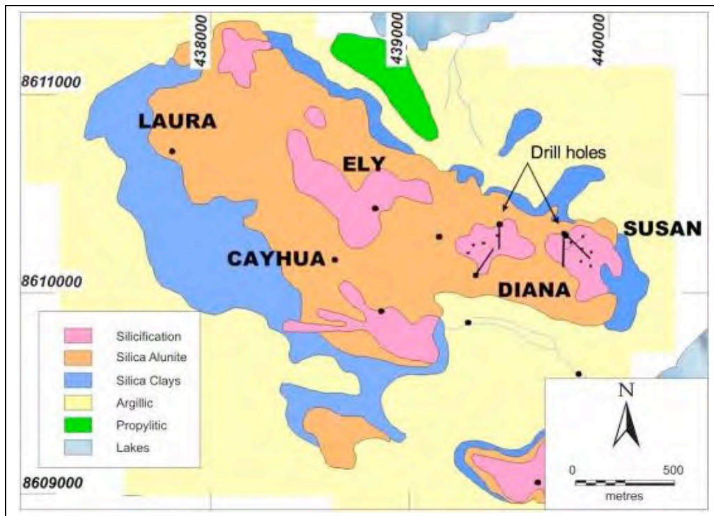
Figure 12 Corihuarmi Project – Main Block Alteration
