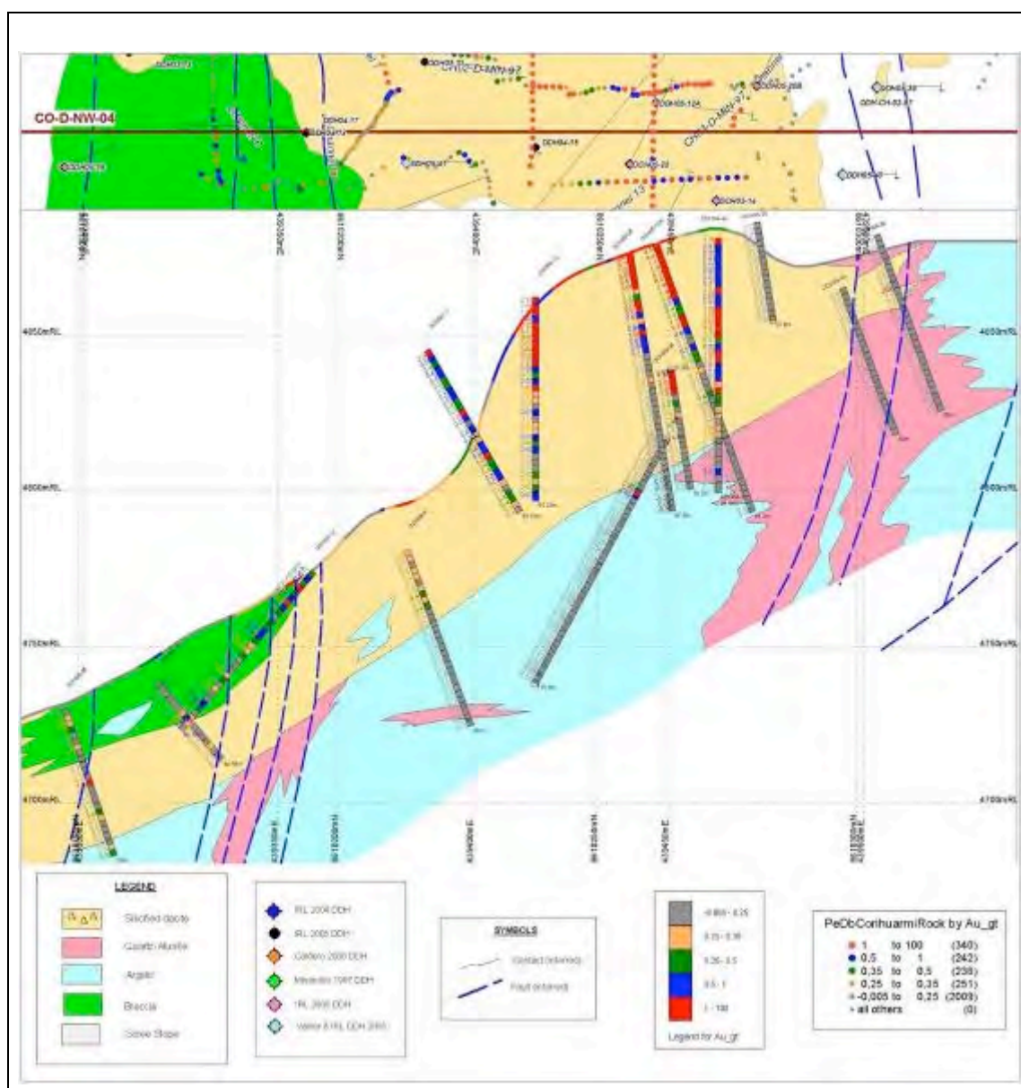
Figure 9 Corihuarmi Project - Diana Deposit – Representative Drill Section
