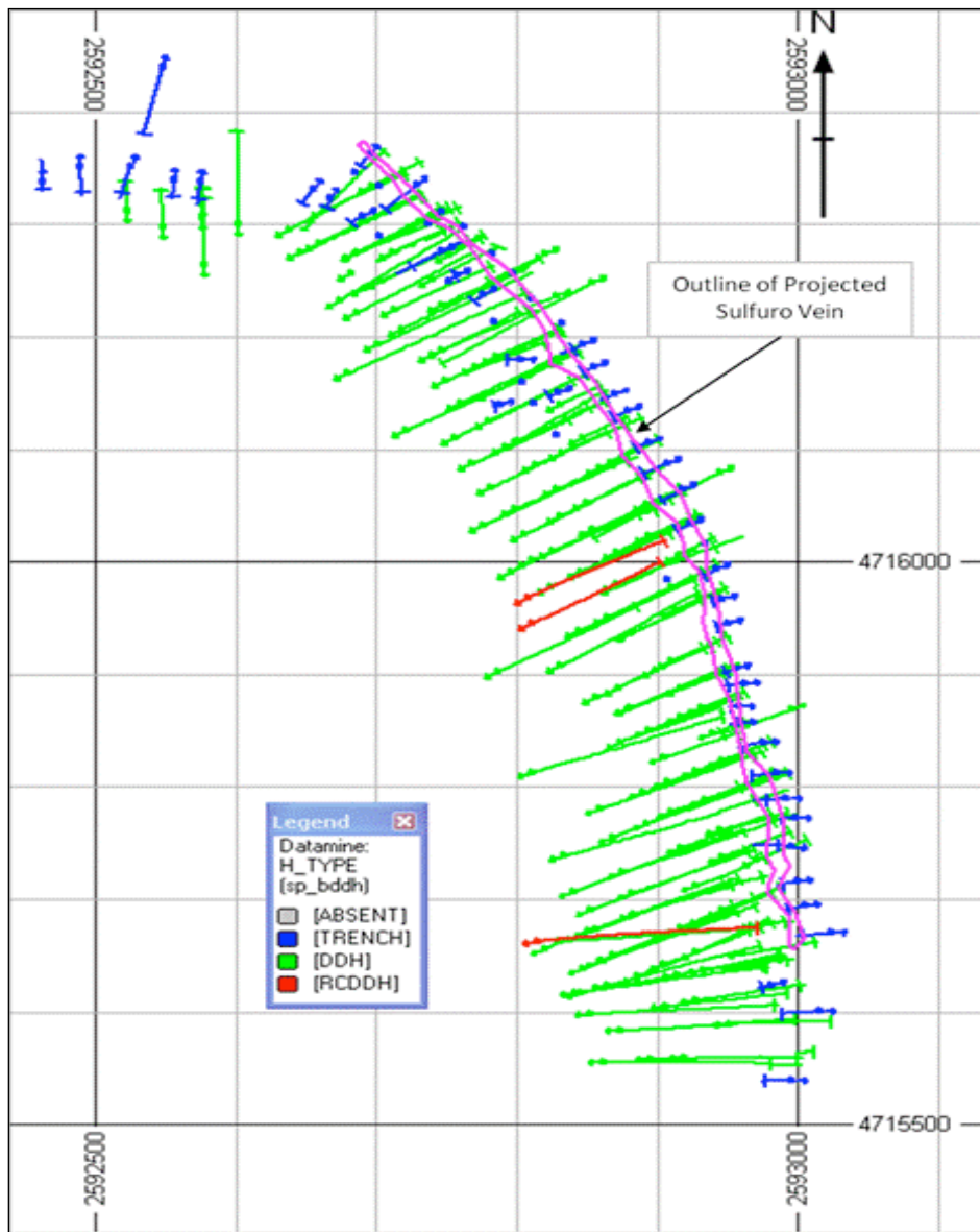
Figure 39 Paloma (Sulfuro) Drill and Trench Plan
