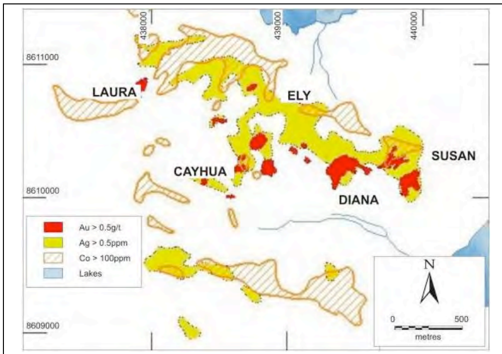
Figure 13 Corihuarmi Project – Main Block Metallogenic Zonation
