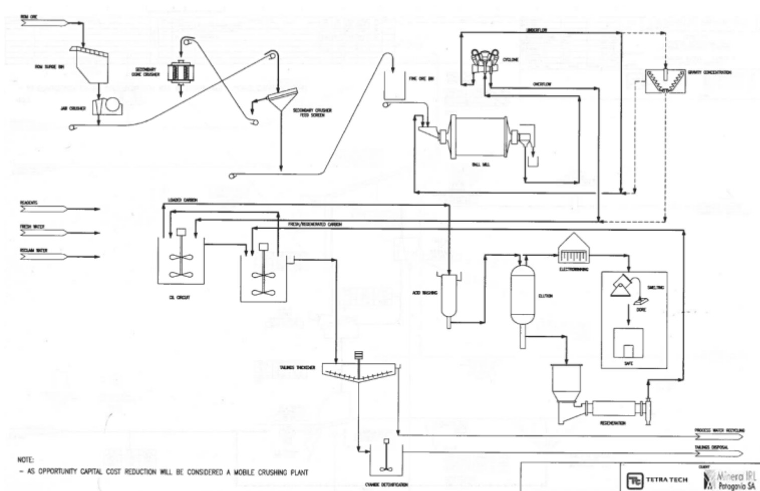
Figure 44 Simplified Process Flowsheet
