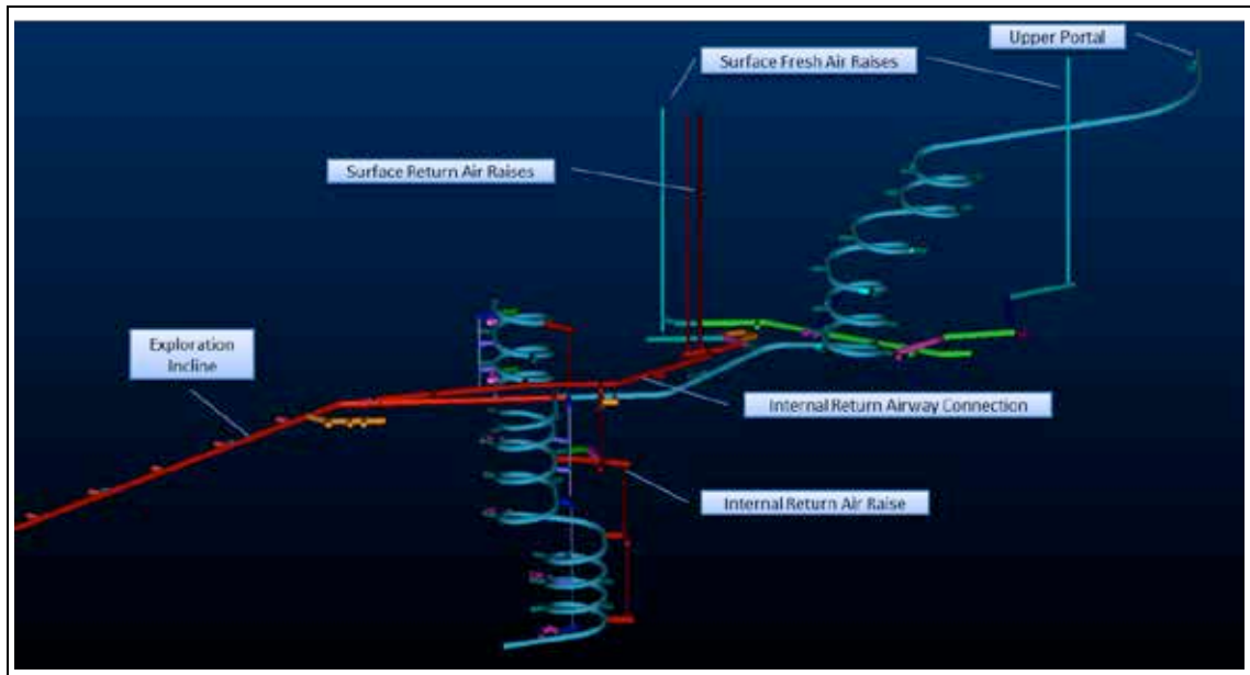
Figure 27 Primary Ventilation System
