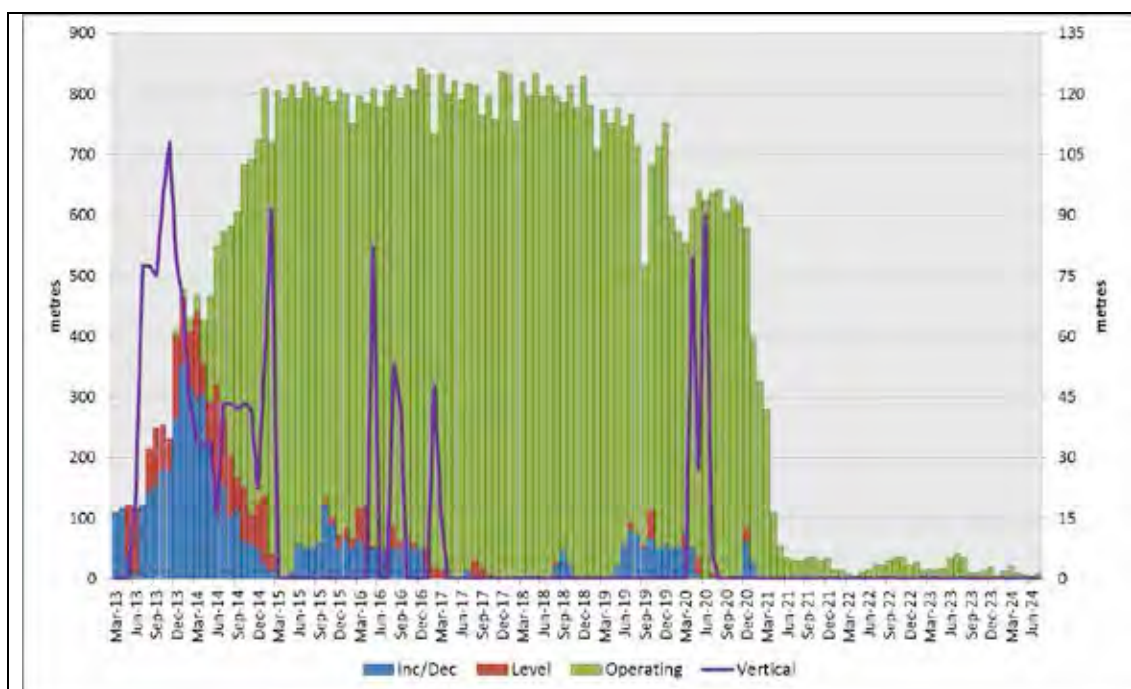
Figure 28 Lateral Development Metres per Month
