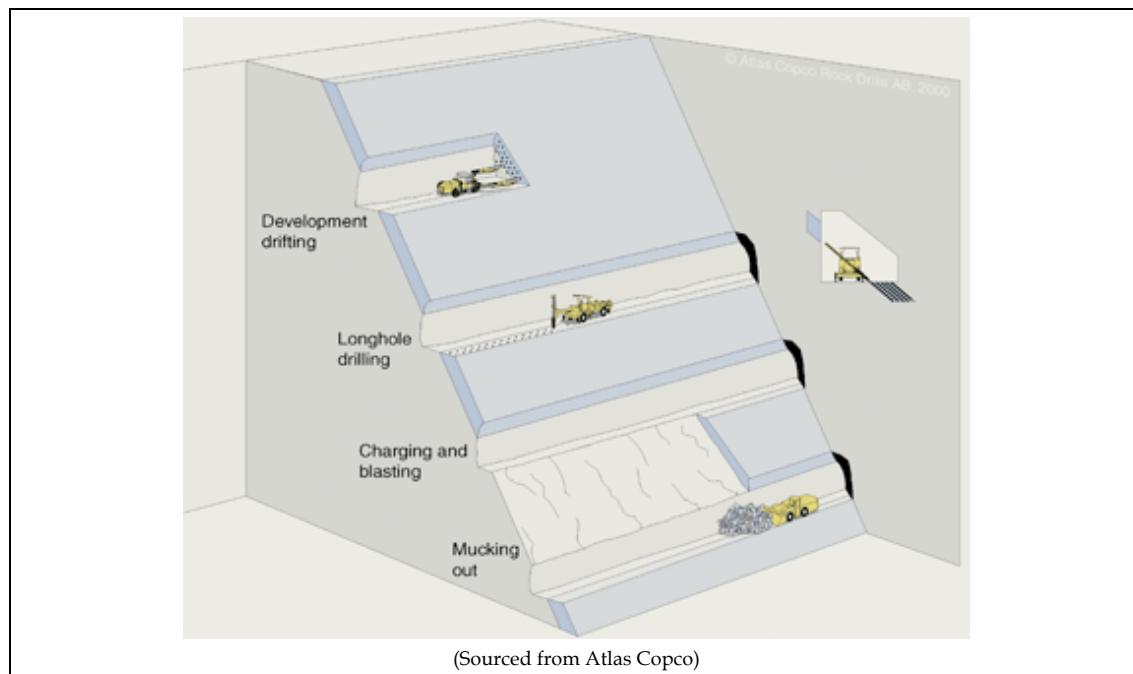
Figure 24 Typical View of the Selected Longitudinal Mining Method
