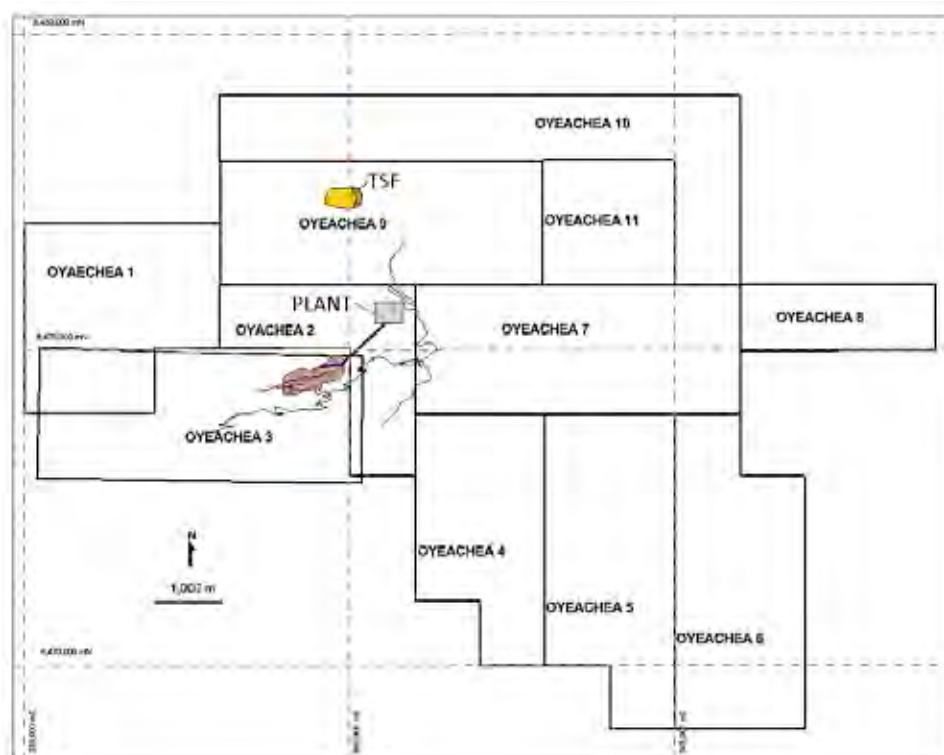
Figure 16 Ollachea Exploration Concession Map
