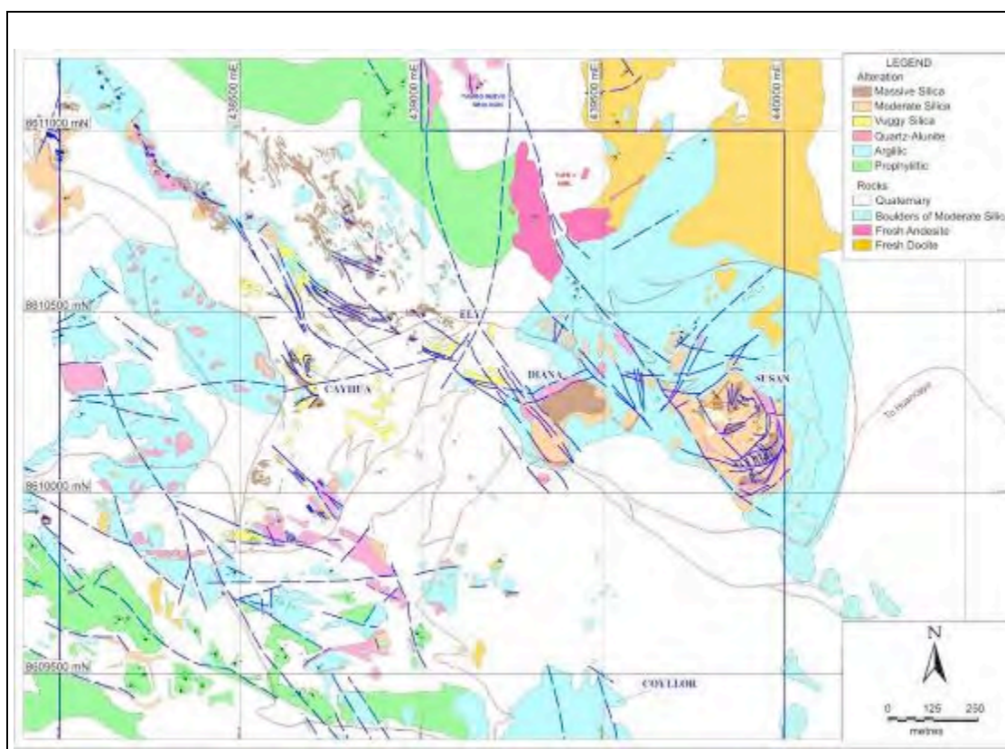
Figure 4 Corihuarmi Project – Geology
