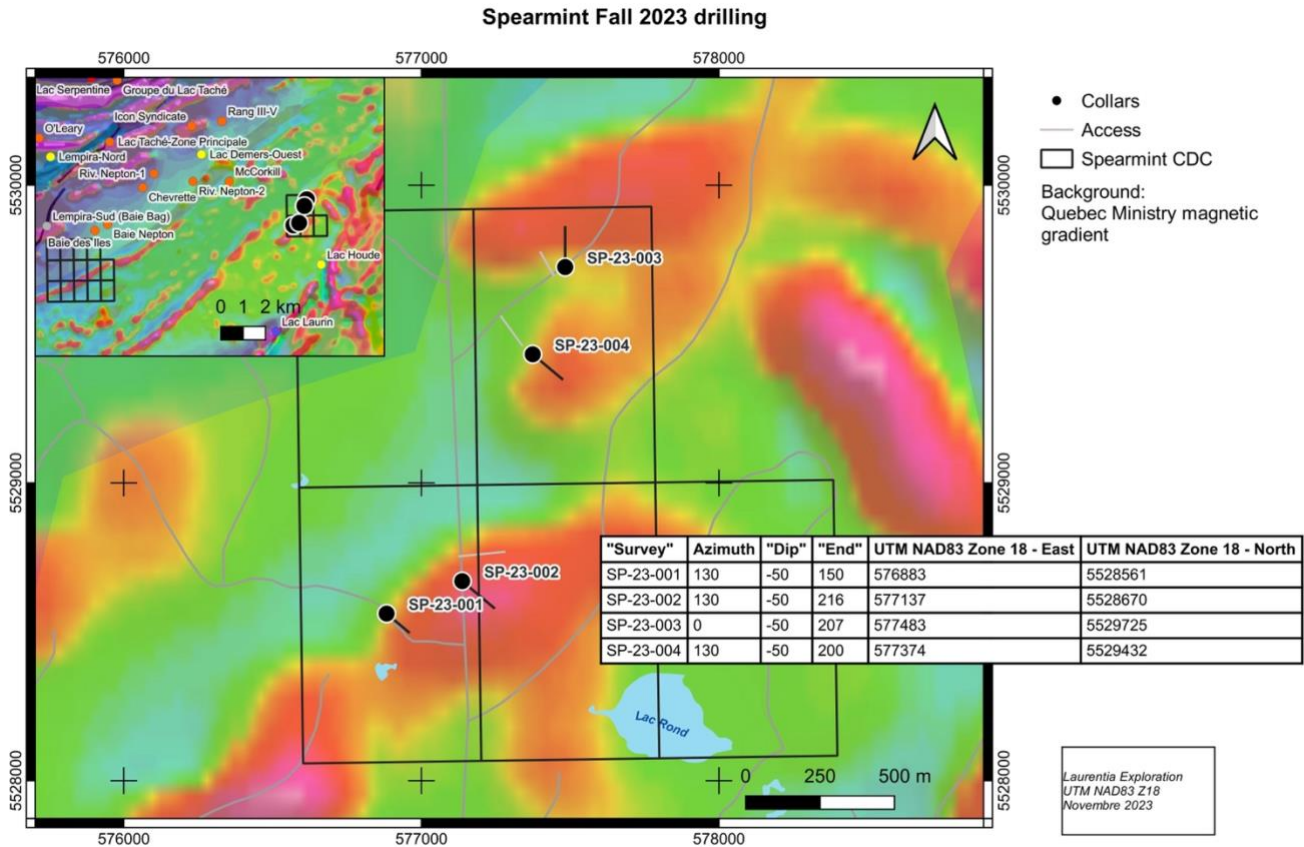
Figure 1: Location of the planned drillholes, access, claims and vertical gradient of the residual magnetic field.
