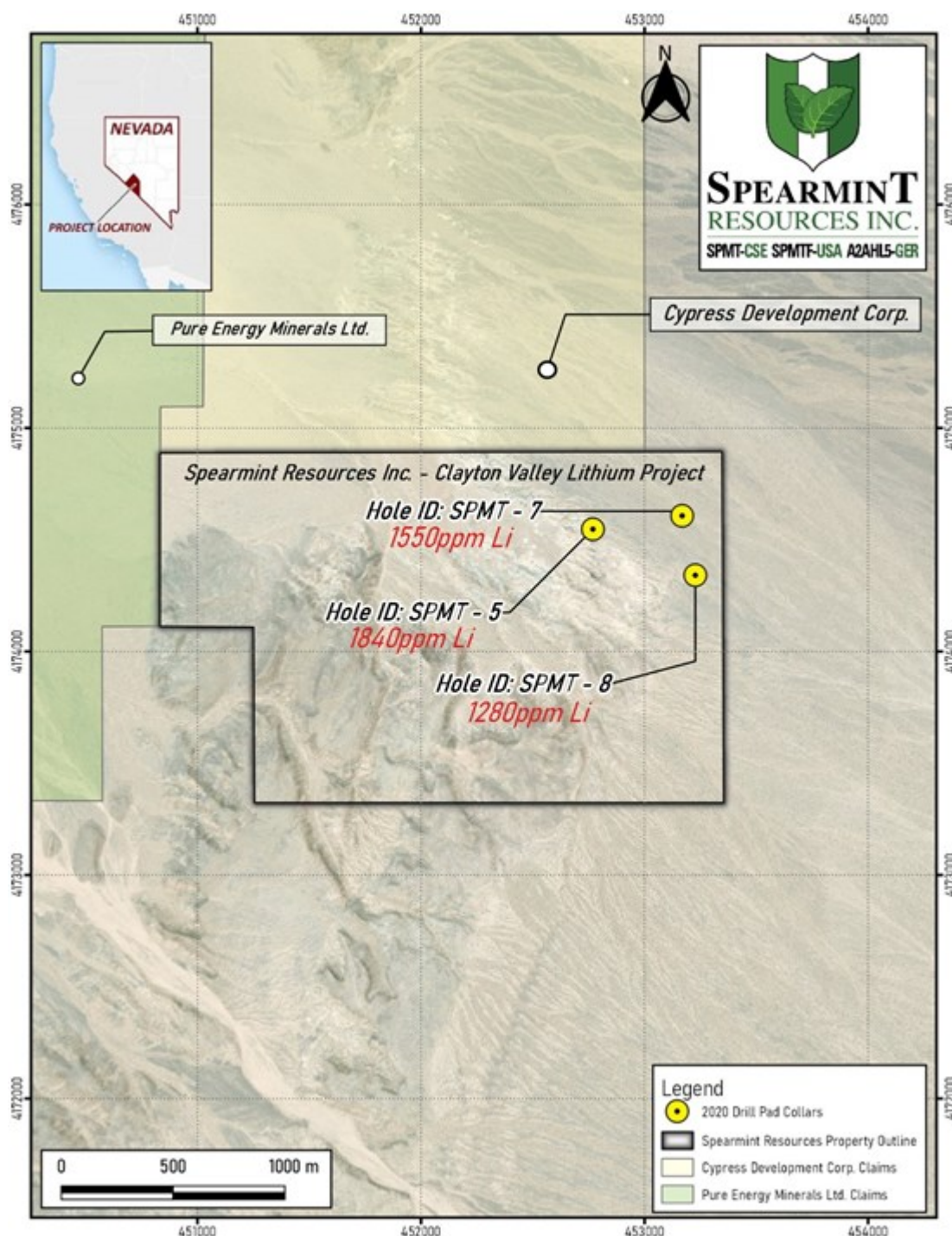
Figure 2: Lithium Values from Spearmint's First 3 Drill Holes of the 2020 Drill Program
