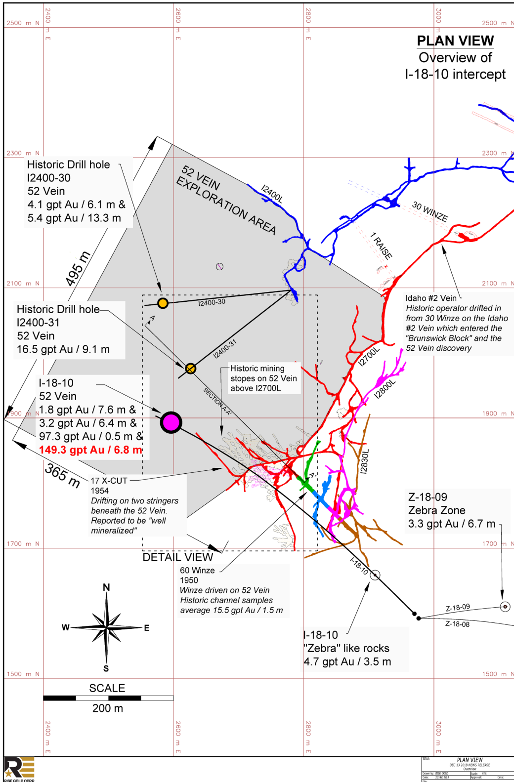
FIGURE 1 – 52 Vein Intercept – Plan View
