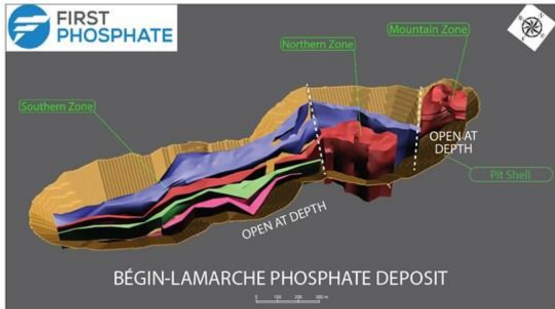
Figure 1 - The Bégin-Lamarche Deposit Pit-Shell
