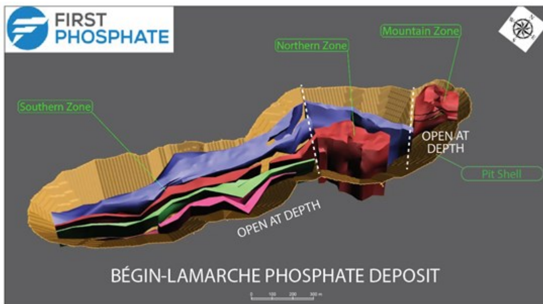
Figure 1 - The Bégin-Lamarche Deposit Pit-Shell
