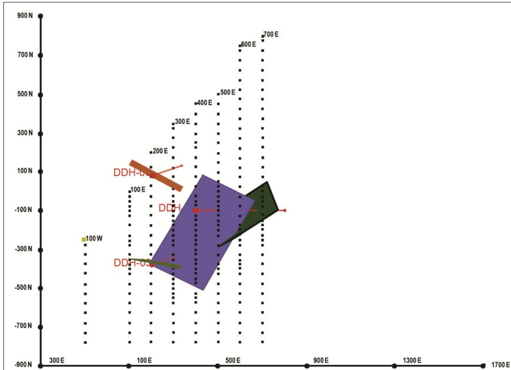
Plan view of the modelled conductors as well as tracing of the suggested drillings.
