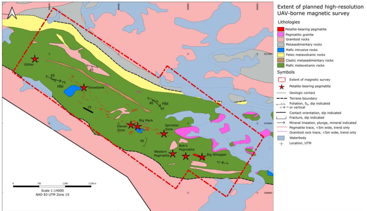
Figure 1 - Planned UAV Magnetic Survey
