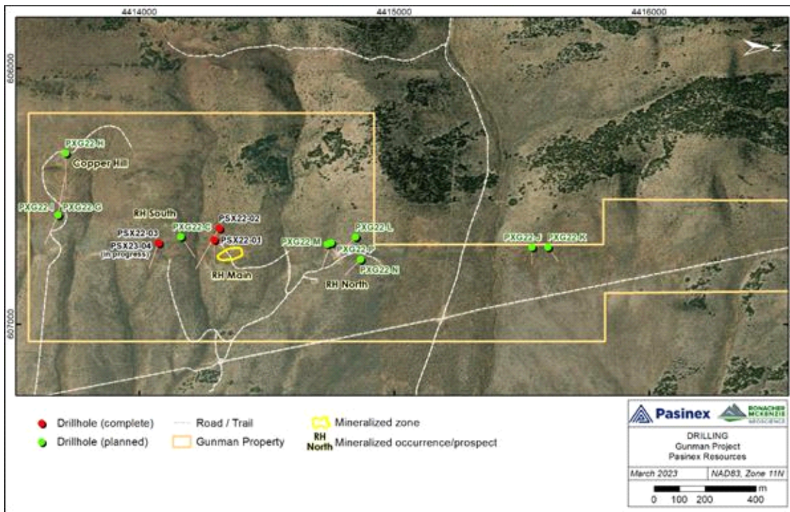
Figure 1 – 2022-2023 planned drilling at the Gunman property. Completed drill holes are indicated with red collars and numbered suffixes. Pending drill holes are indicated with green collars and letter suffixes. RH Main zinc mineralized zone and other mineralized prospects are shown along a two-kilometre trend.
