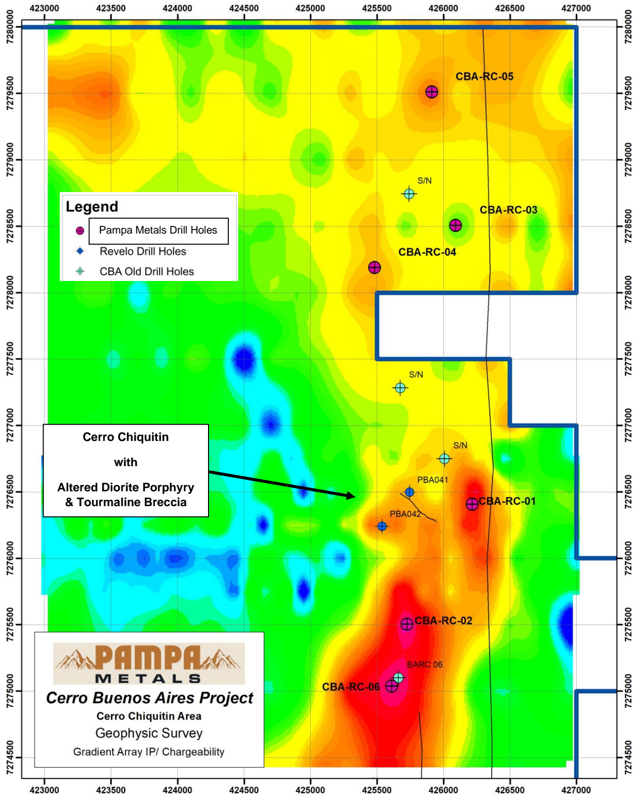
Cerro Buenos Aires – Cerro Chiquitin Area – Gradient Array IP Chargeability and Drill Holes
