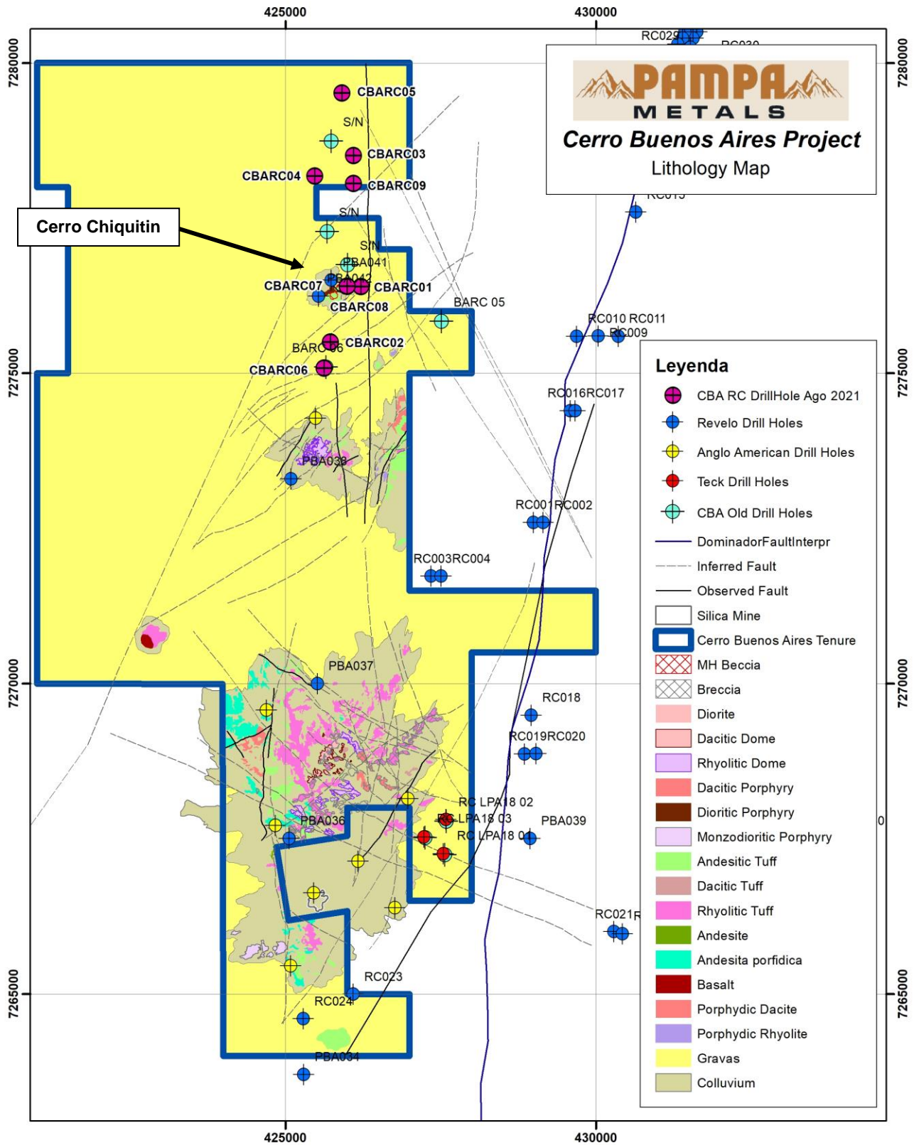
Cerro Buenos Aires - General Geology Map Showing Historic Drilling and New Drill Holes
