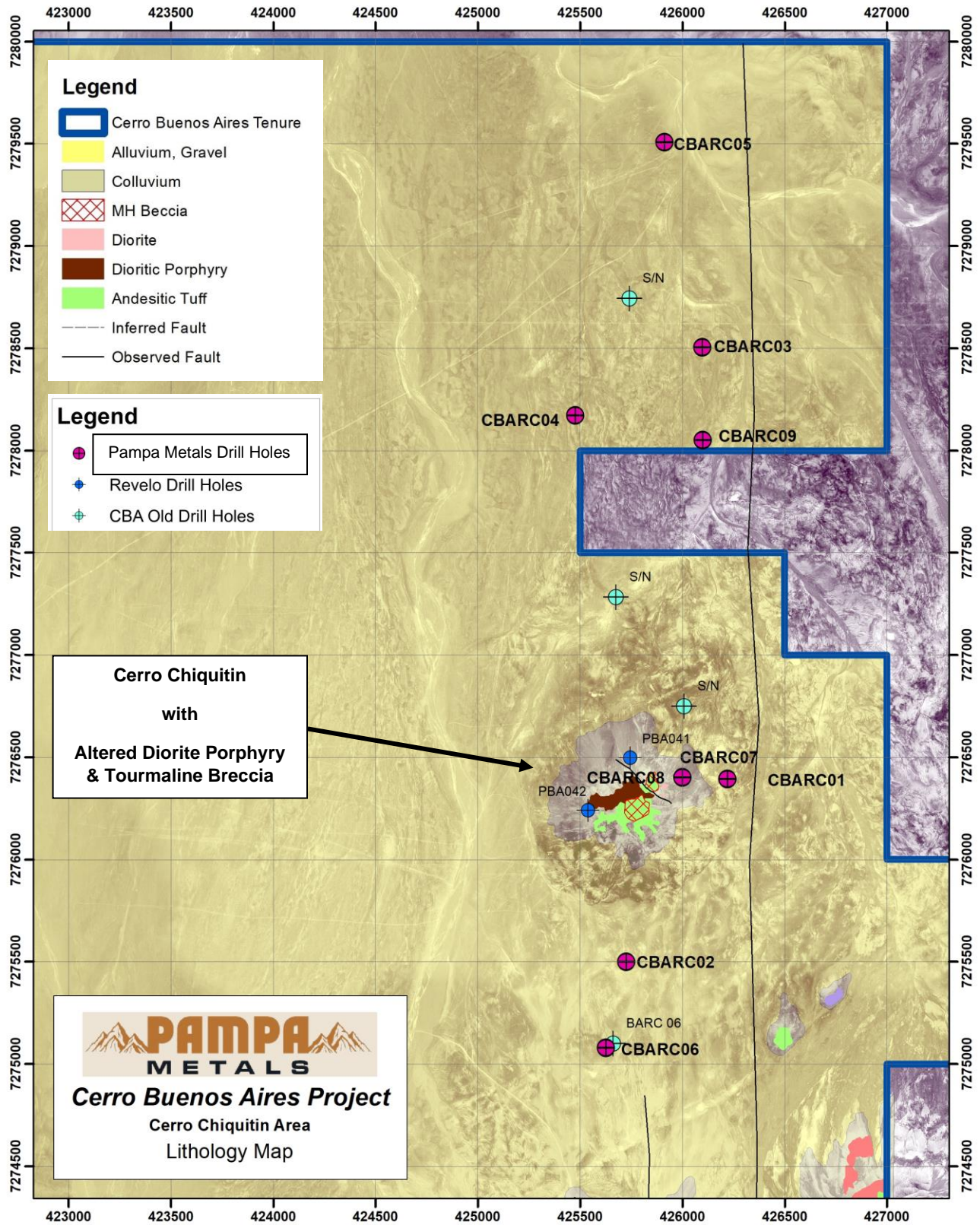
Cerro Buenos Aires – Cerro Chiquitin Area – Showing Simplified Geology and Drill Holes
