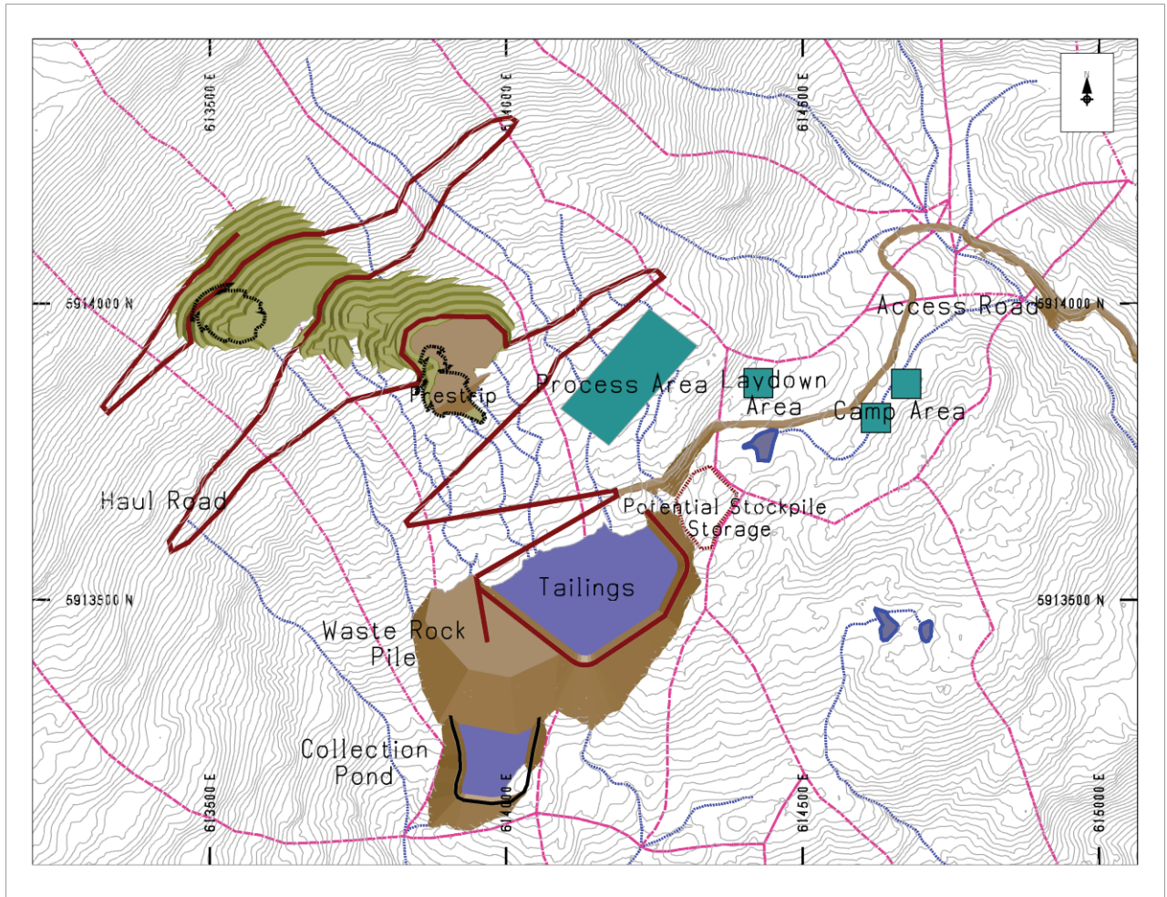
Figure 16-21 EOP 10 Mine Layout
