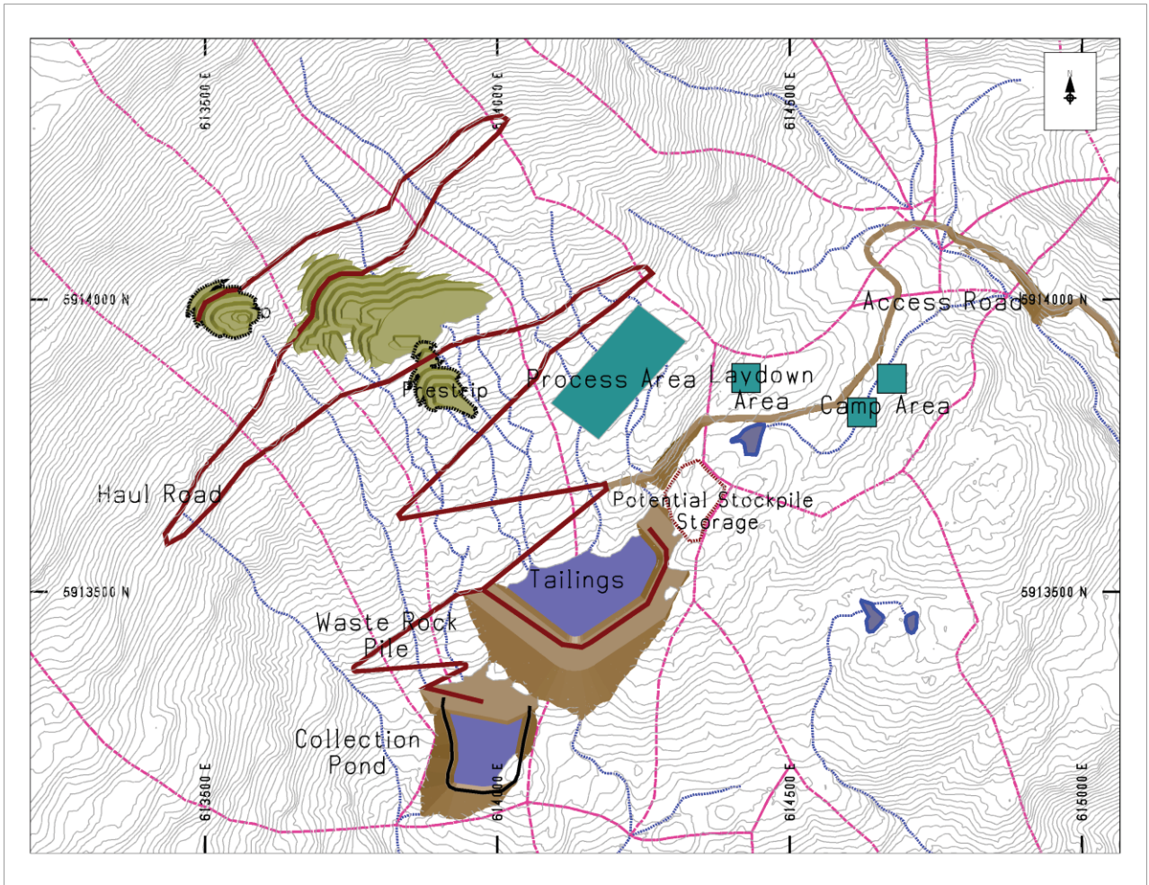
Figure 16-19 EOP 04 Mine Layout
