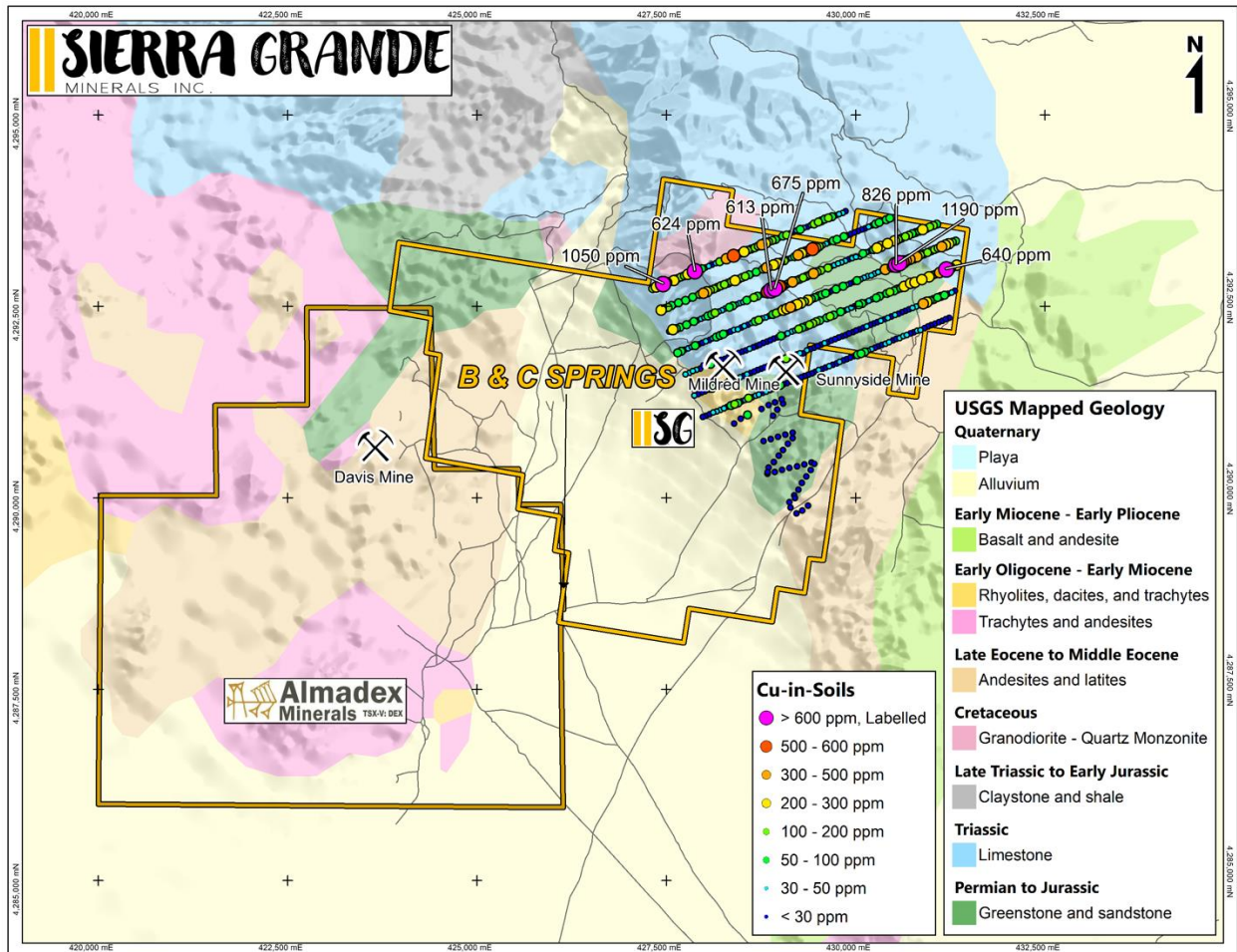
Figure 3. B&C Springs-Mildred regional setting with Copper-in-soil results
