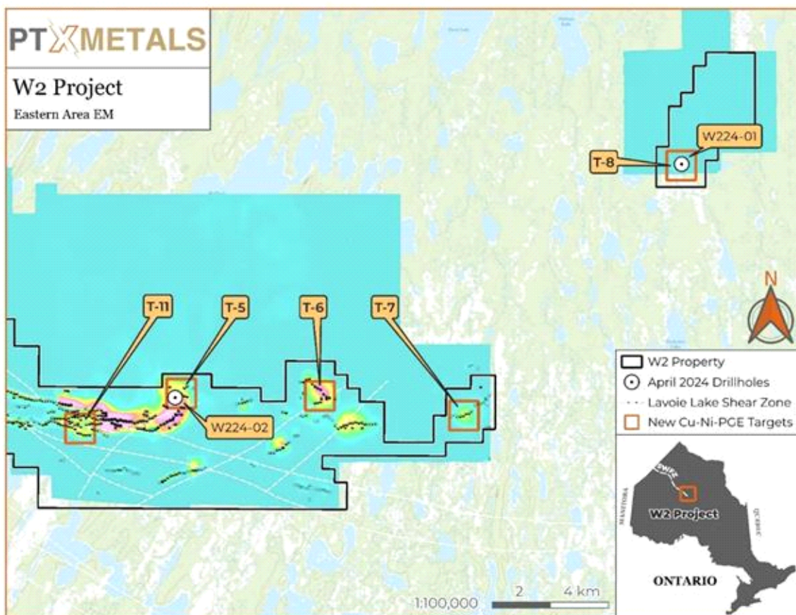
Figure 2: Plan View of 2024 Drill Holes in the W2 Eastern Area
