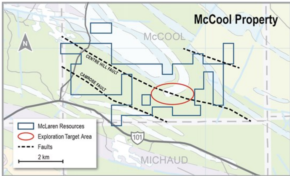
Map 1 - The favorable target area for gold in relation to the Centre Hill Fault, the sub-parallel Camrose Fault and the McCool Anticline. http://www.mclarenresources.com/mccool.html (figure #3)
